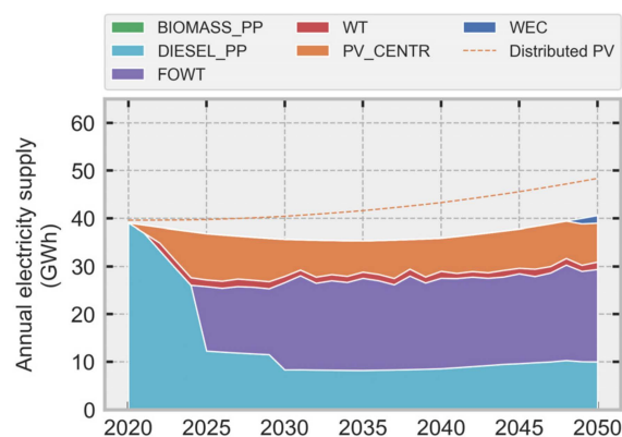
Figure 14. Stack plot representing the annual electricity mix for the High PV, Medium EV scenario.
