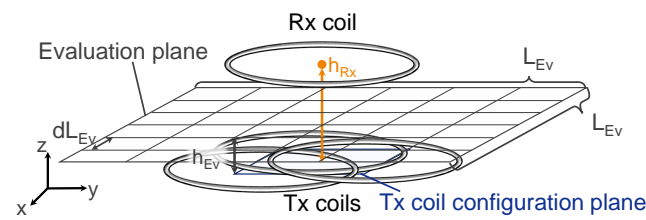
Figure 5. Evaluation points in the evaluation plane.
