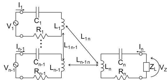
Figure 2. Equivalent circuit of wireless power transfer via magnetic resonance coupling (MRC-WPT) using phased array transmission (Tx) coils. Since the magnetic field at the position of the interfering object was assumed to be suppressed, their effect was ignored (approximation).
