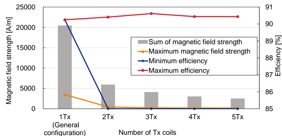
Figure 8. Comparison of magnetic field strength and transmission efficiency for each number of transmission (Tx) coils ( \alpha = 0.9 ).
