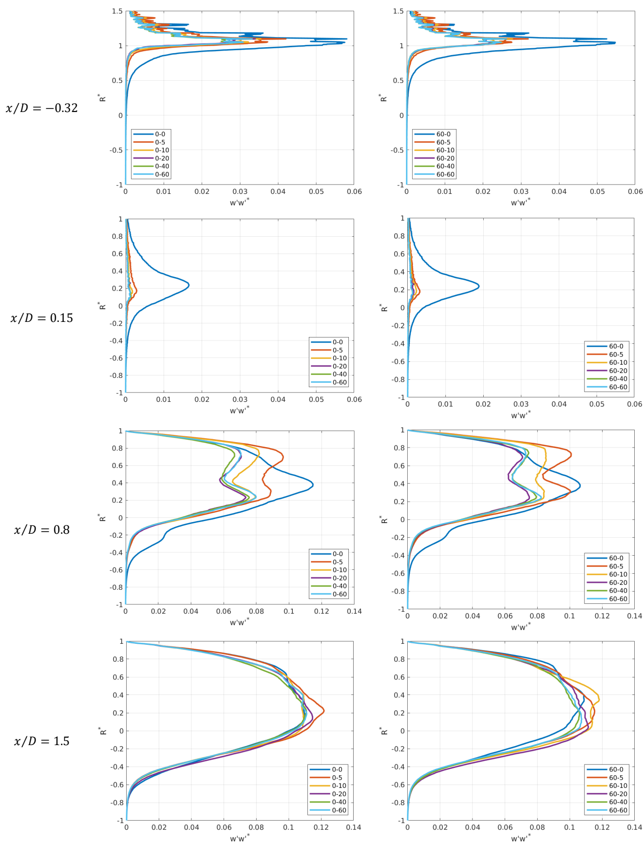
Figure 12. Vertical profiles of w'w'^* at different cross-sections.
