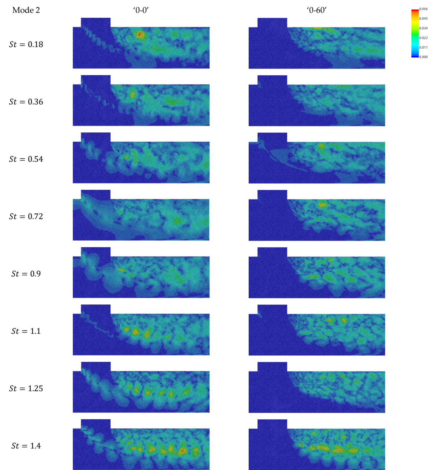
Figure 24. Contour plots of mode 2 of in-plane velocity vector coloured by mode magnitude for XZ plane.
