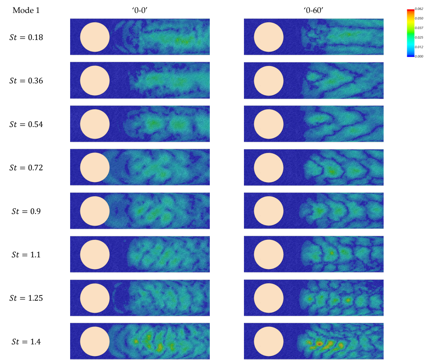
Figure 25. Contours plots of mode 1 of in-plane velocity vector coloured by mode magnitude for XY plane.
