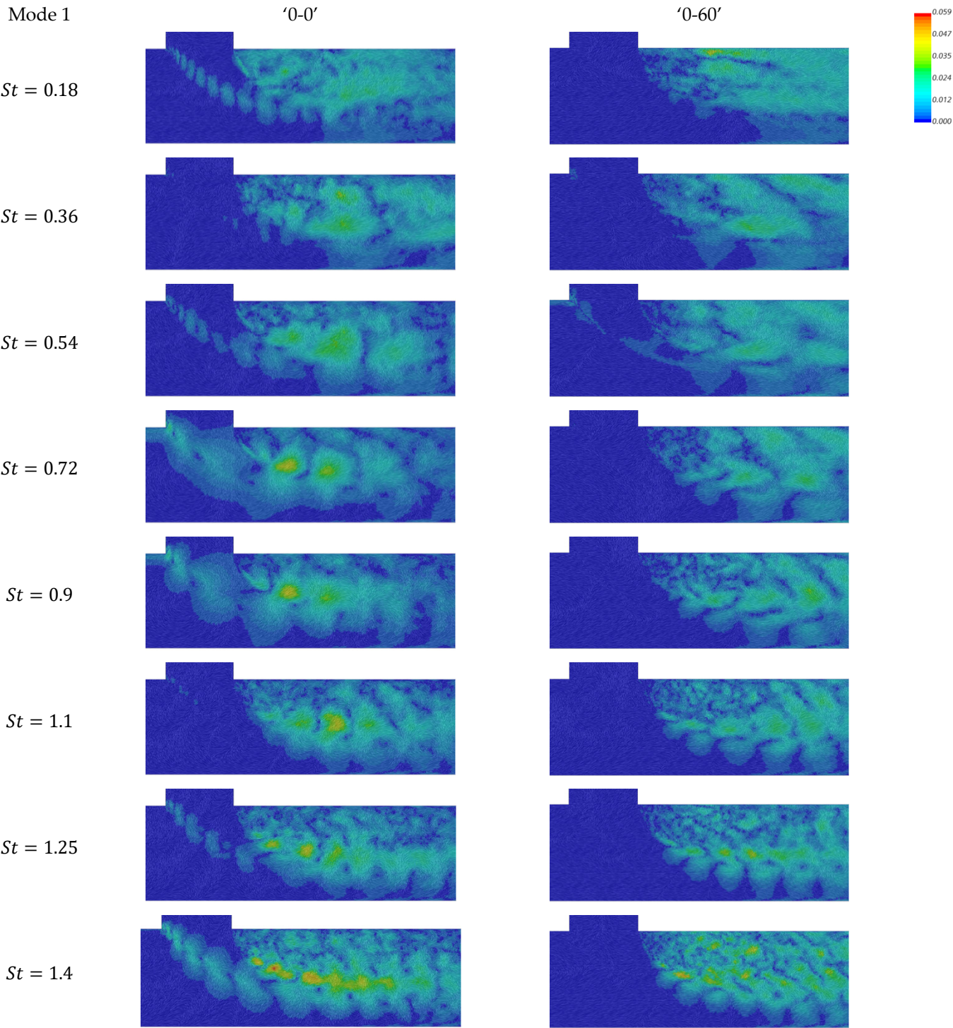
Figure 23. Contour plots of mode 1 of in-plane velocity vector coloured by mode magnitude for XZ plane.
