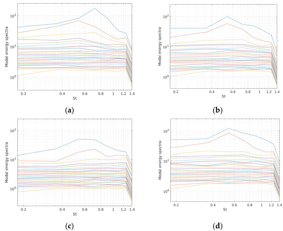
Figure 22. Modal energy spectra for case '0-0' of x-component (a) and y-component (c) of velocity and for case '0-60' x-component (b) and y-component (d) of velocity on XY symmetry plane. The different colour lines represent the different modes.
