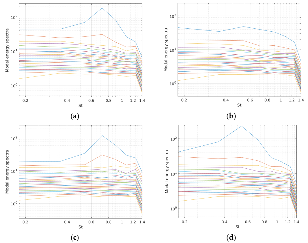
Figure 21. Modal energy spectra for case '0-0' of x-component (a) and z-component (c) of velocity and for case '0-60' x-component (b) and z-component (d) of velocity on XZ symmetry plane. The different colour lines represent the different modes.
