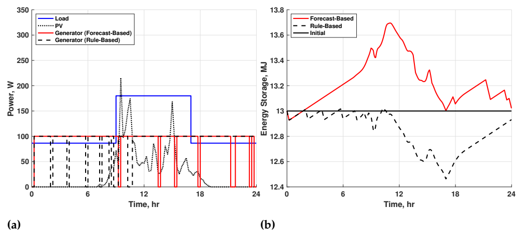
Figure 6. Stress case 1 power (a) and energy storage (b).
