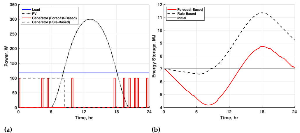
Figure 5. No stress case power (a) and energy storage (b).
