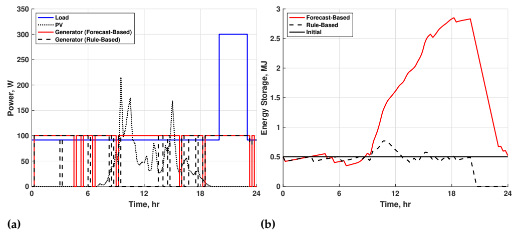
Figure 7. Stress case 2 power (a) and energy storage (b).
