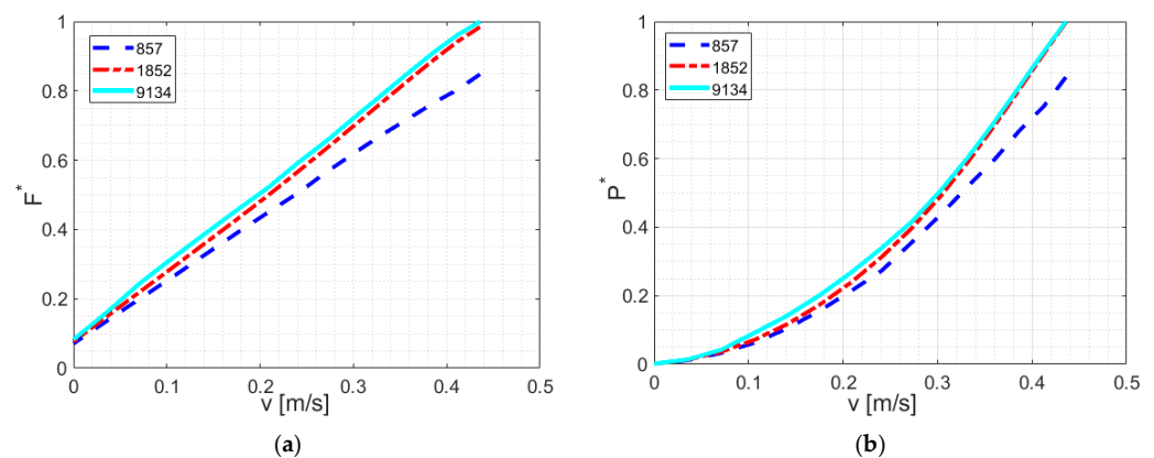
Figure 5. Mesh sensitivity with an increasing overall number of finite elements (curve parameter): (a) normalised damping force vs. piston speed; (b) normalised harvested power vs. piston speed.
