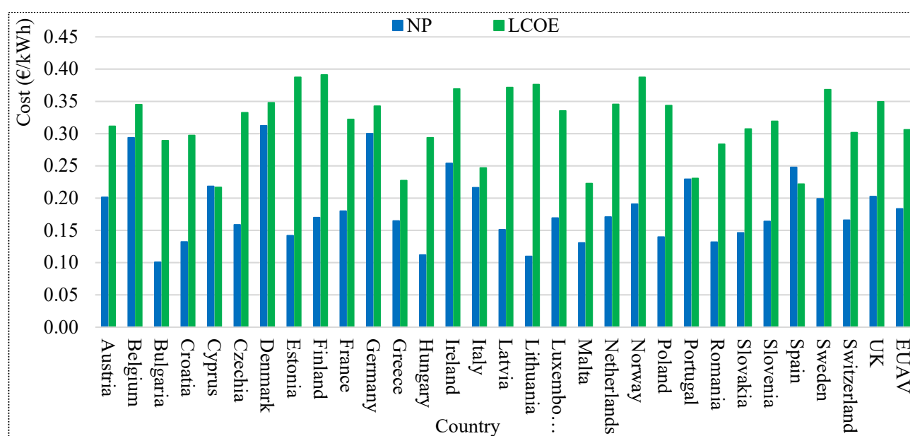
Figure 8. NP and LCOE of a non-optimal solution.
