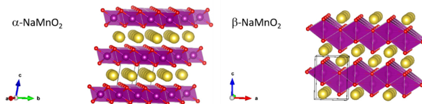
Figure 1. Representations of the structure of the two polymorphs of NaMnO 2 (red = oxygen atoms; purple = MnO 6 octahedra; yellow = sodium atoms).
