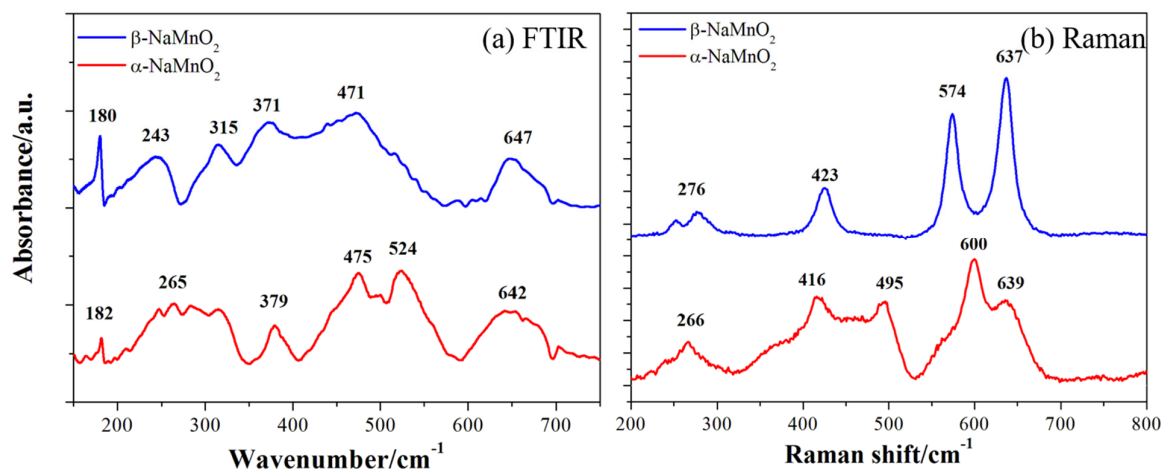
Figure 6. (a) Fast Fourier Transform Infrared spectroscopy (FTIR) and (b) Raman spectra of the \alpha -NaMnO 2 and \beta -NaMnO 2 phases.
