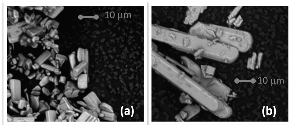
Figure 3. Scanning electron microscopy (SEM) micrographs of the as-synthesized samples: (a) \alpha -NaMnO 2 ; (b) \beta -NaMnO 2 .
