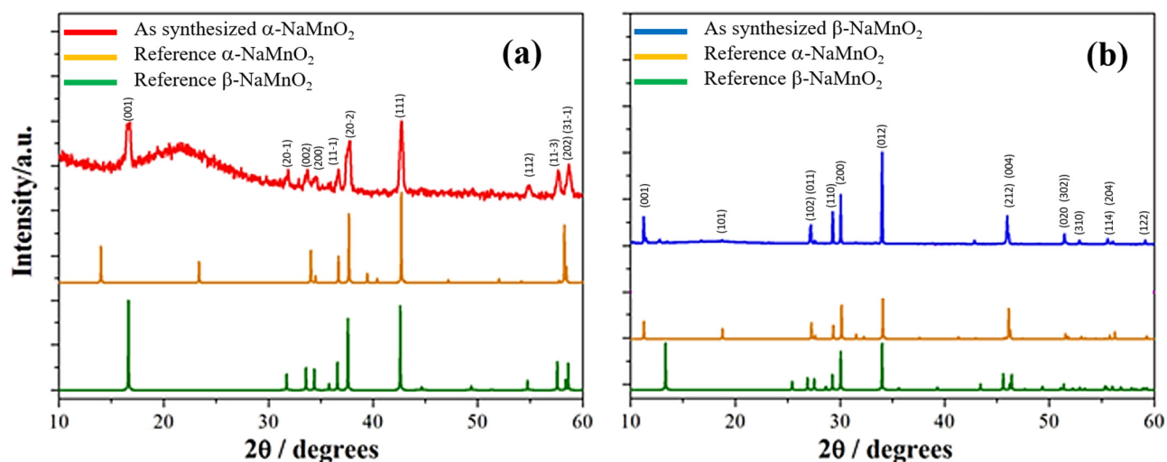
Figure 2. X-ray diffraction (XRD) patterns of the as-synthesized samples: (a) \alpha -NaMnO 2 conventional XRD ( \lambda = 1.54 \text{ \AA} ); (b) \beta -NaMnO 2 synchrotron radiation XRD ( \lambda = 1.24 \text{ \AA} ).
