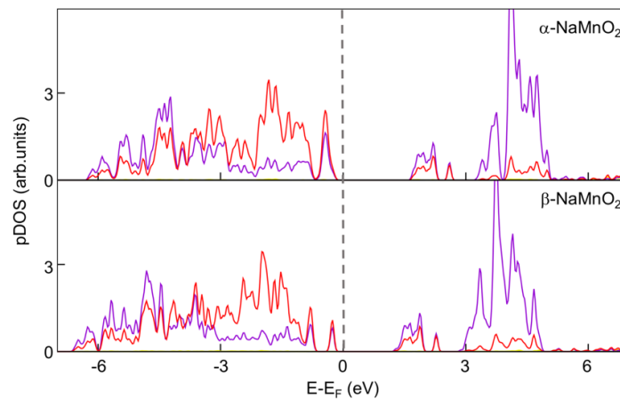
Figure 5. Atom- and angular momentum- projected density of states (pDOS) computed for \alpha -NaMnO 2 ( top ) and \beta -NaMnO 2 ( bottom ) at PBE+U-D3BJ level of theory. Color code: Mn d (purple), O p (red).
