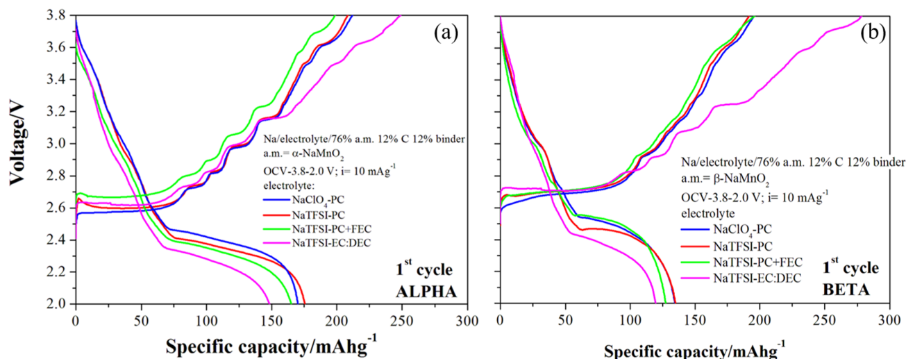
Figure 7. Charge/discharge voltage profiles during galvanostatic tests of the (a) \alpha - \text{NaMnO}_2 and (b) \beta - \text{NaMnO}_2 phases.
