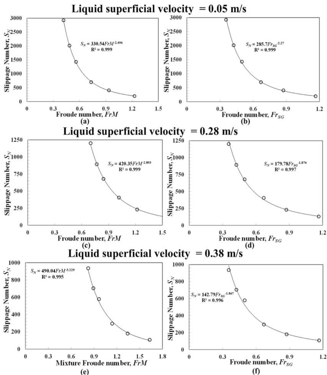
Figure 15. Correlation of Slippage Number ( S_N ) with either Froude Number ( Fr_{SG} ) or Mixture Froude Number ( FrM ) for upward flows. System fluid: air–silicone oil. Flow pattern under consideration: Slug flow. Liquid superficial velocity of (a) 0.05 m/s, (b) 0.05 m/s, (c) 0.28 m/s, (d) 0.28 m/s, (e) 0.38 m/s, and (f) 0.38 m/s.
