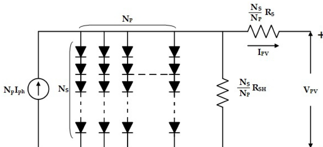
Figure 3. Equivalent circuit of a PV array.
