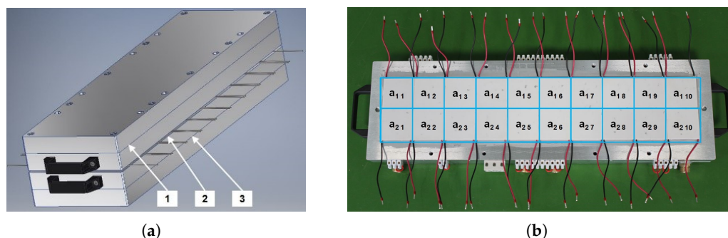
Figure 5. MTEG view with arrangement of individual TEGs; (a) model (1—hot side exchanger, 2—TEG layer, 3—cold side heat exchanger); (b) hot side exchanger prototype with THM.
