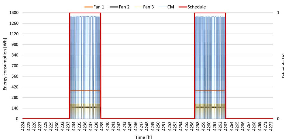
Figure 11. Energy consumption. DX system in Lampedusa in two representative summer days.
