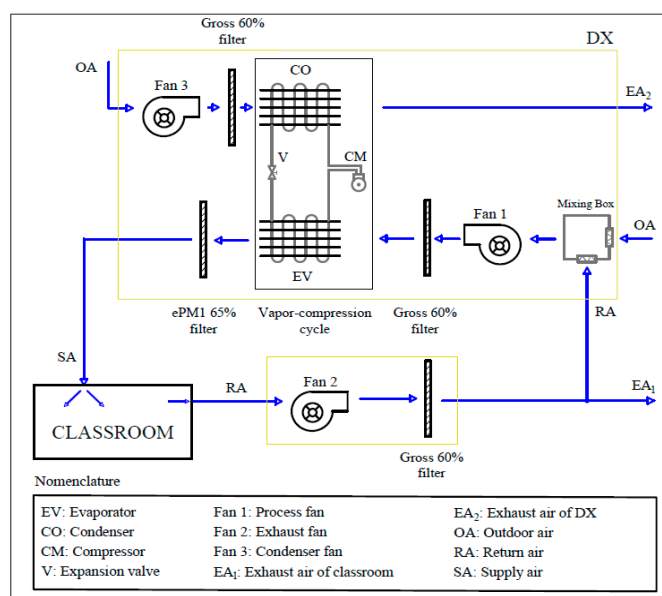
Figure 1. Schematic of the DX system.
