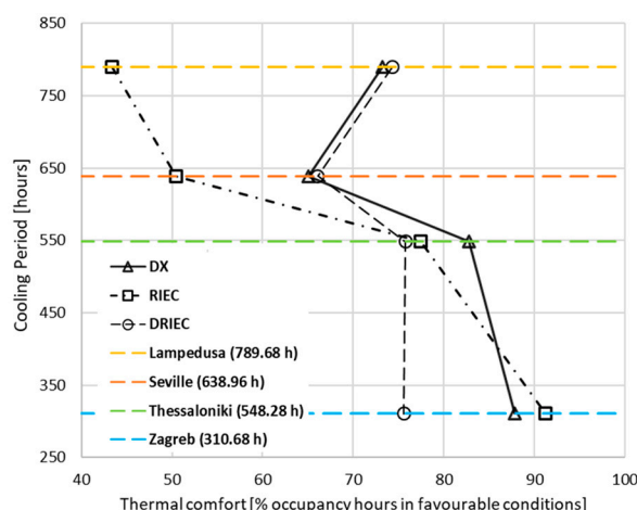
Figure 16. Influence of climatic severity on thermal comfort indicator.
