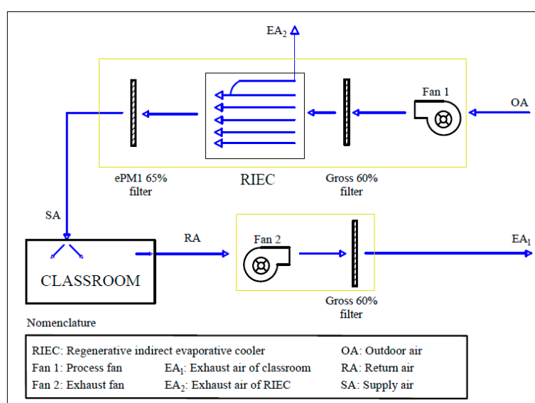
Figure 2. Schematic of the RIEC system.
