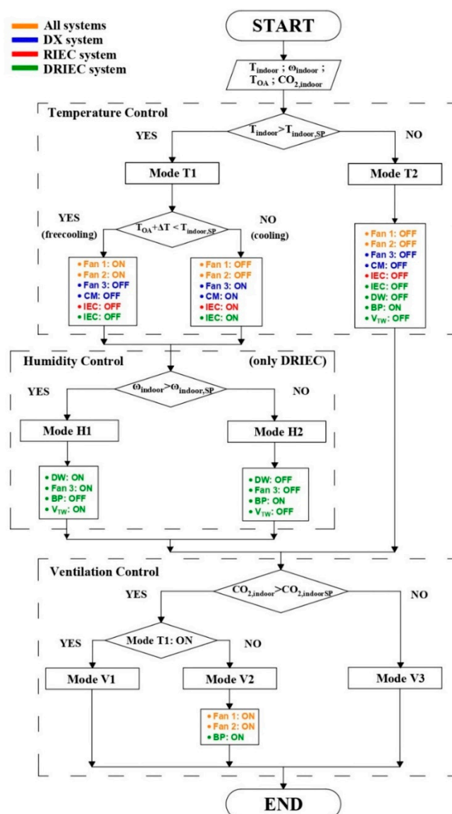
Figure 4. Air-cooling systems control logic diagram.
