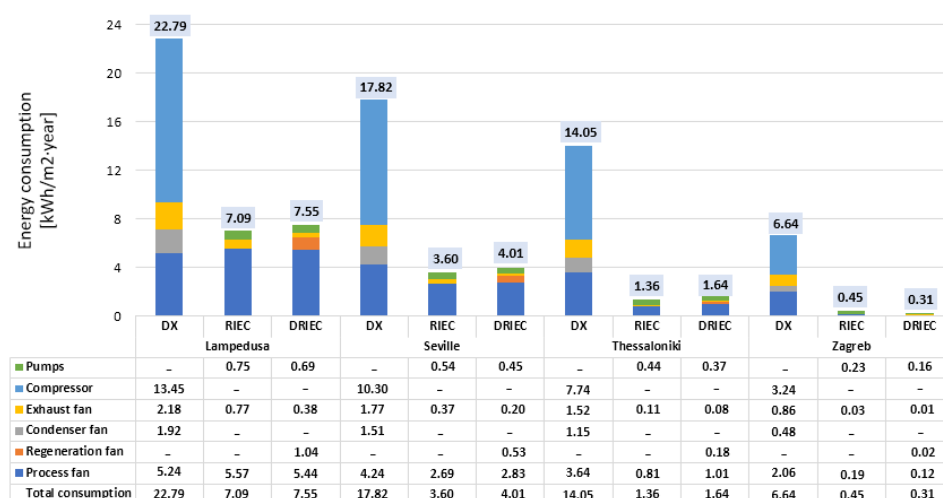
Figure 14. Annual energy consumption results.
