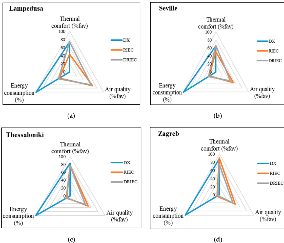
Figure 19. Radar chart. Systems and climate zones comparison (a) Lampedusa; (b) Seville; (c) Thessaloniki and (d) Zagreb.
