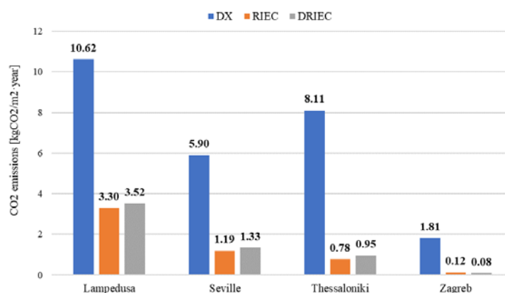
Figure 15. Annual CO 2 emissions results.
