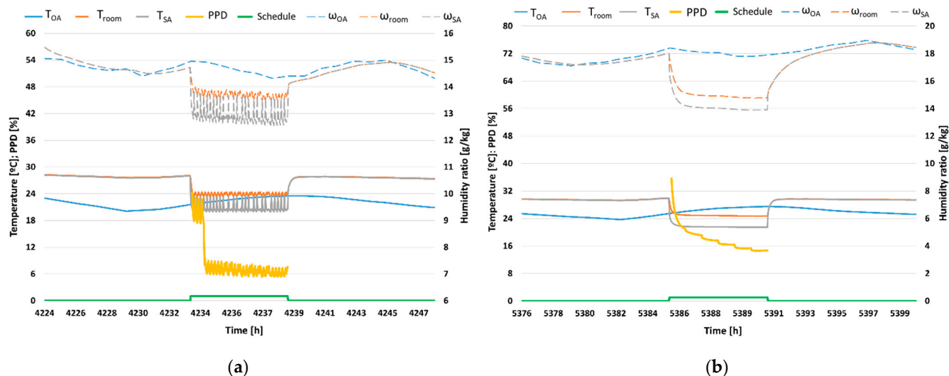
Figure 5. Temperature and humidity. DX system in Lampedusa. (a) Typical summer day and (b) Severe summer day.
