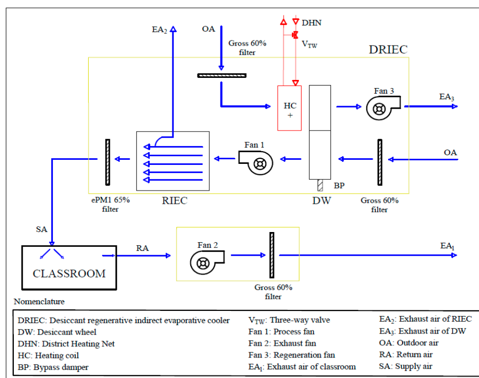
Figure 3. Schematic of the DRIEC system.
