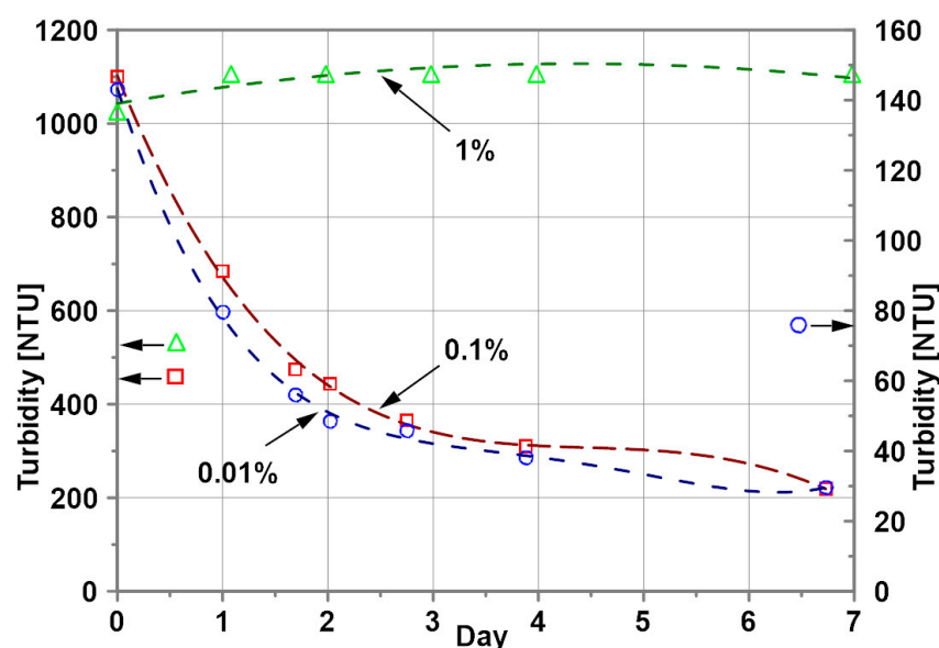
Figure 4. Turbidity of water–Al 2 O 3 nanofluids; nanoparticle concentration: ○ - 0.01%, □ - 0.1%, △ - 1%.
