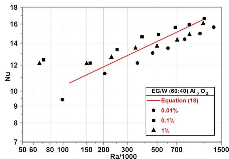
Figure 8. Nu–Ra relationship for EG/water (60/40) mixture-based nanofluids.
