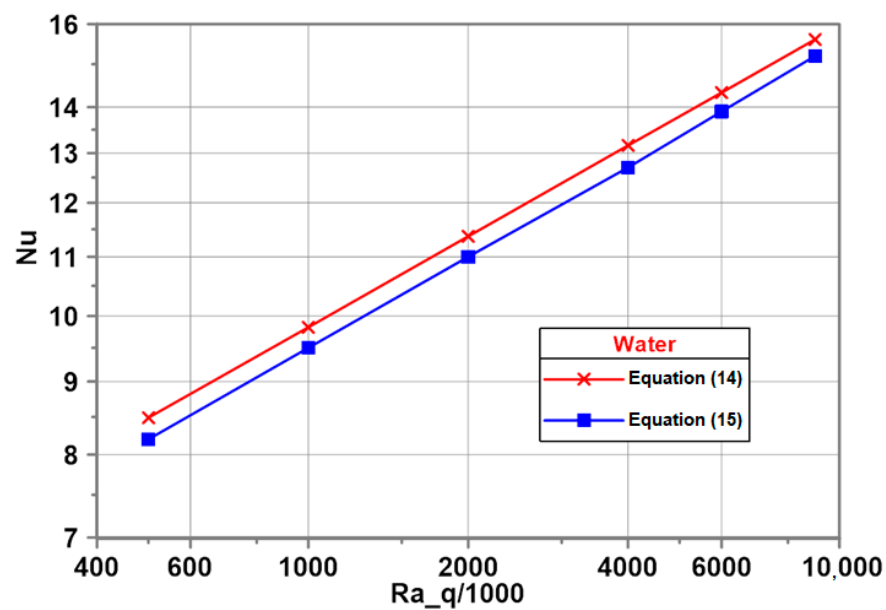
Figure 5. Present data compared to predictions from the literature correlation.
