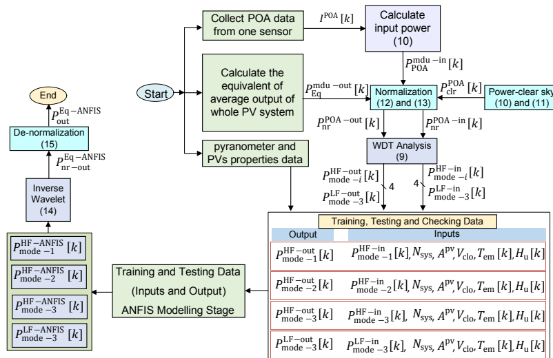
Figure 2. Proposed methodology for the proposed ANFIS– DWT technique.
