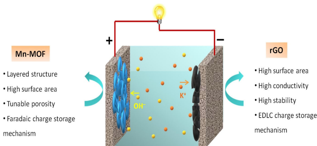
Figure 6. Schematic illustration of hybrid supercapacitor with Mn-MOF as a positive electrode and rGO as a negative electrode in KOH aqueous electrolyte [32].
