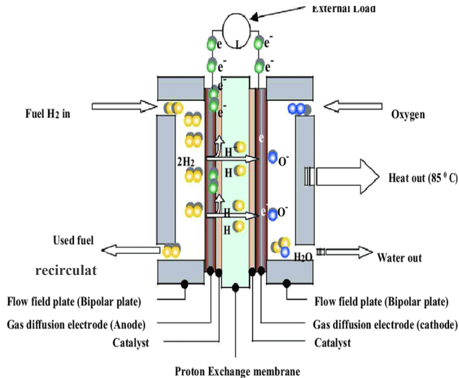
Figure 13. Schematic of working principle of polymer electrolyte membrane fuel cell [150].
