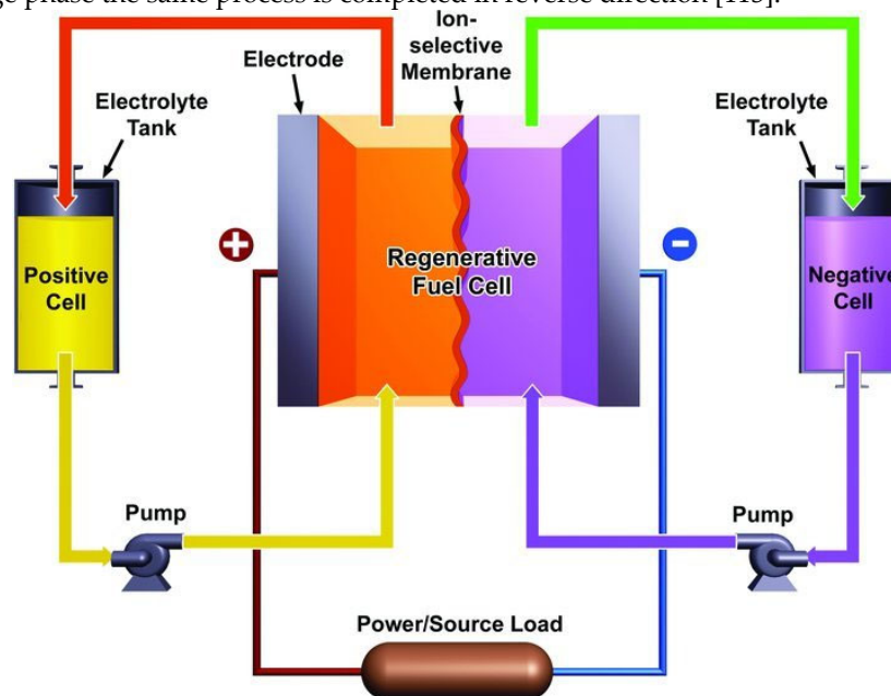
Figure 10. Schematic representation of a redox flow battery [114].
