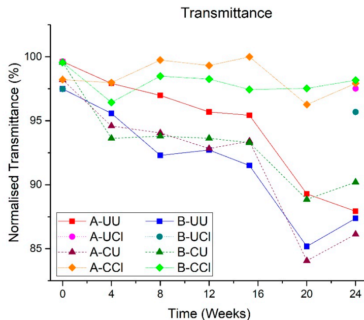
Figure 9. Reduction in normalised transmittance for coated and uncoated A and B is shown as a function of outdoor exposure time. Abbreviations: UU—Uncoated uncleaned, UCl—Uncoated cleaned, CU—Coated uncleaned, CCl—Coated cleaned.
