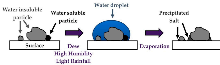
Figure 12. Illustration of the cementation process adapted from Cuddihy [20] and Ilse et al. [18].
