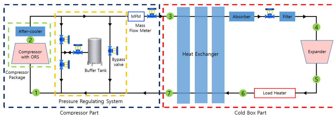
Figure 3. Schematic diagram of the proposed reverse Brayton cryogenic system. ORS: oil removal system.
