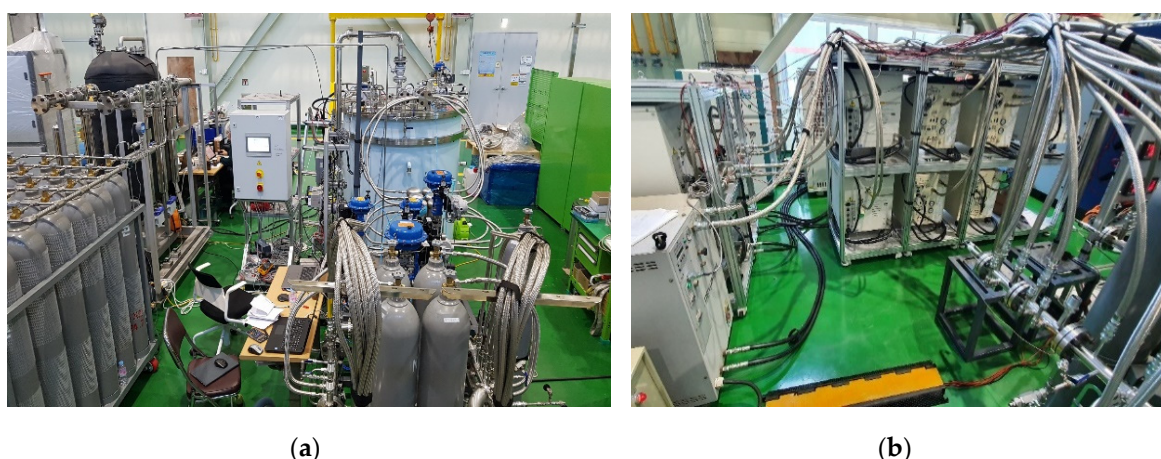
Figure 4. The constructed reverse Brayton cryogenic system: (a) cold box and pressure regulating system (PRS) and (b) compressor package.
