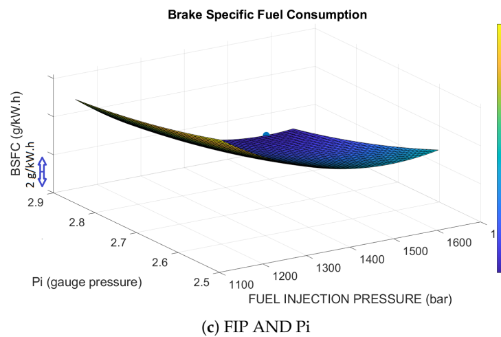
Figure 8. Response surface of the BSFC at one operating point.
