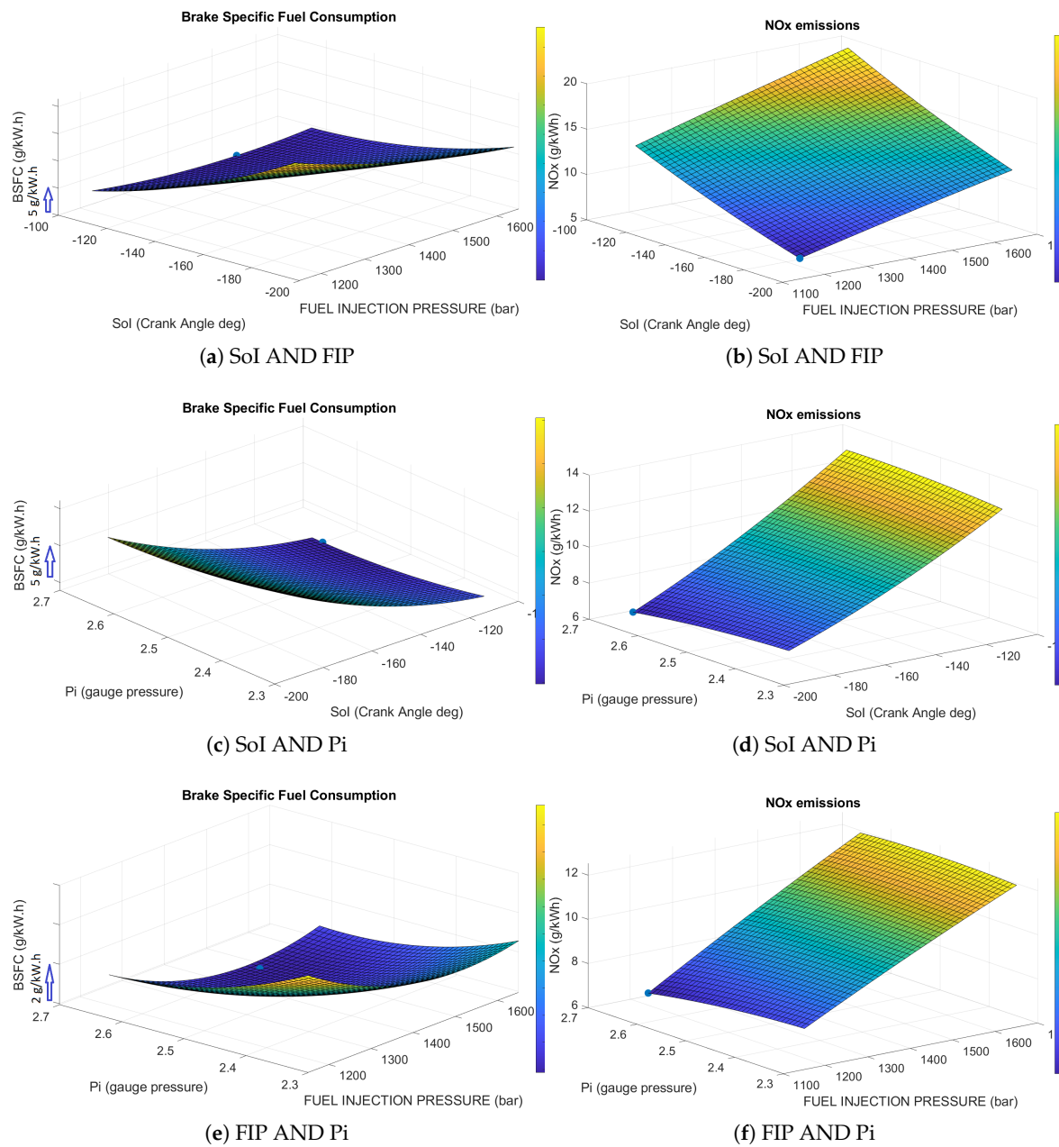
Figure A3. Response surface of the BSFC & \text{NO}_x at 1000 RPM-600kW.
