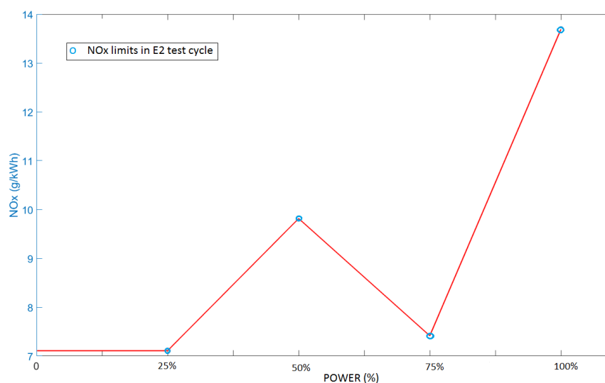
Figure 3. IMO E2 test cycle.
