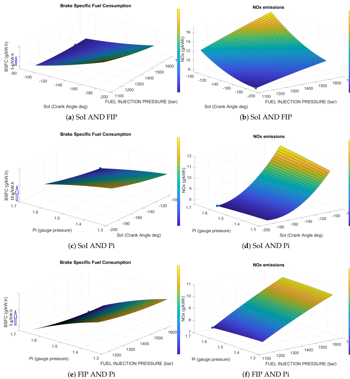
Figure A2. Response surface of the BSFC & \text{NO}_x at 1000 RPM-400kW.
