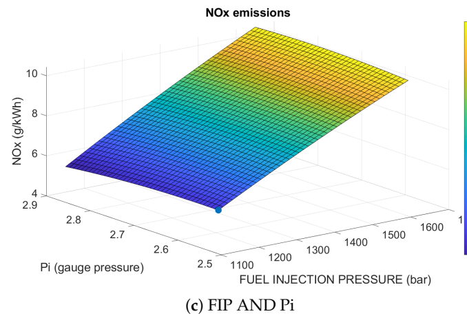
Figure 9. Response surface of the NO_x at one operating point.
