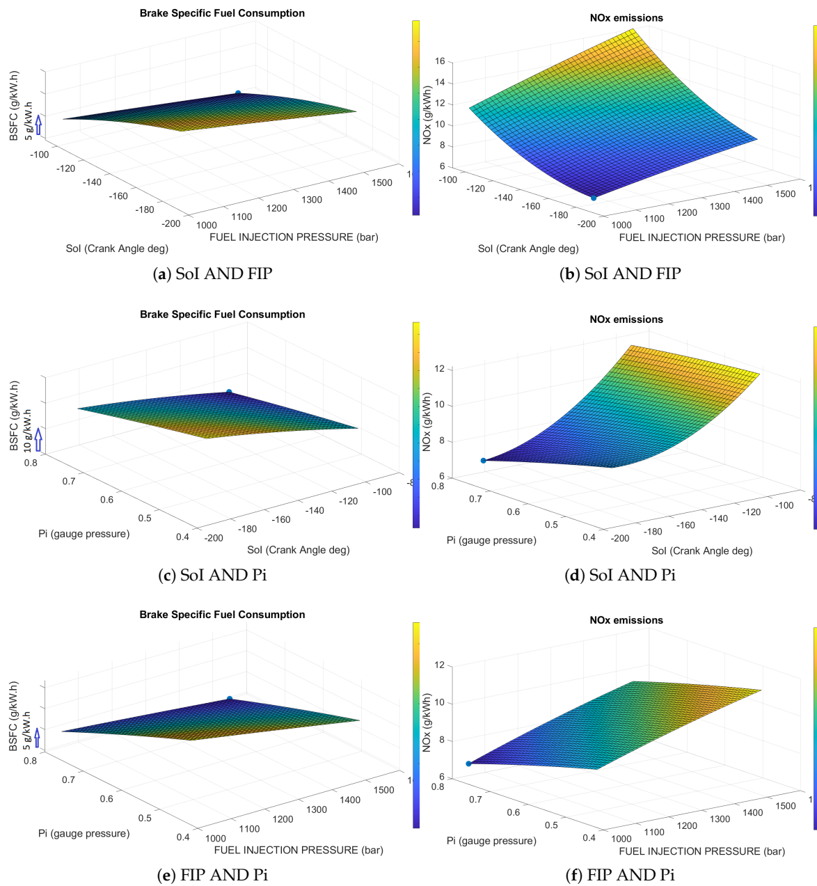
Figure A1. Response surface of the BSFC & \text{NO}_x at 1000 RPM-200kW.
