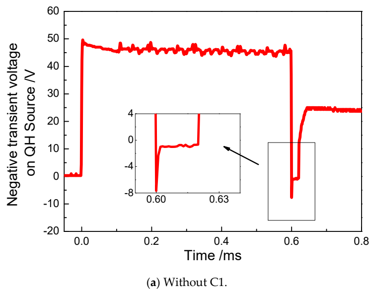
Figure 7. Voltage spike in the variable freewheeling drive circuit.
