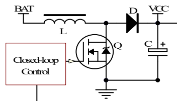
Figure 11. Boost circuitry.
