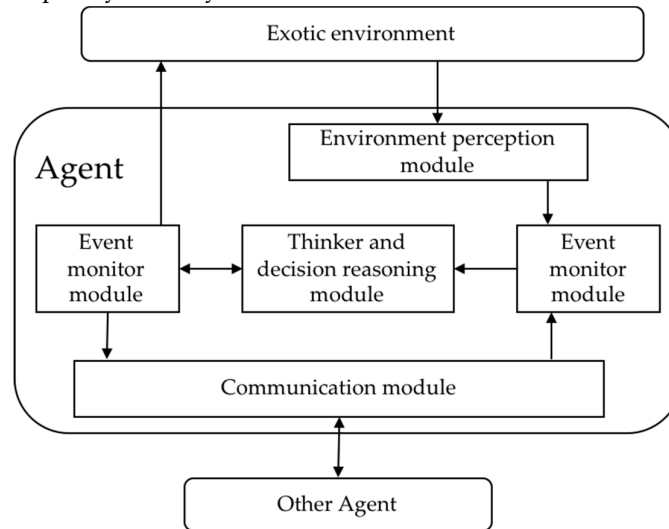
Figure 1. Agent structure [13].
