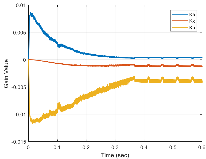
Figure 12. Adaptive gains values; at 1000 W/m 2 , 25 °C and R = 15 \Omega .
