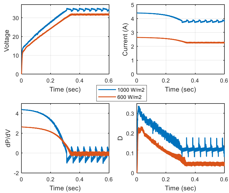
Figure 11. Voltage, current, dP/dV , and D for two irradiance cases; 1000 W/m 2 and 600 W/m 2 at 25 °C and R = 15 \Omega .
