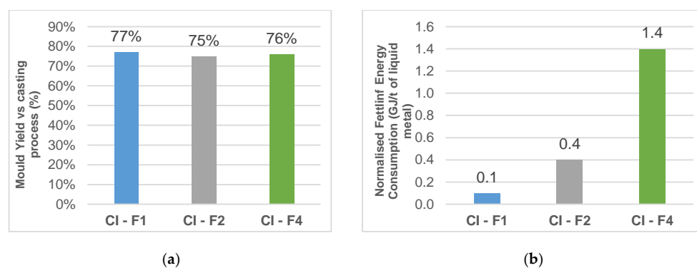
Figure 11. Fettleing process: (a) mold yield in different casting processes; (b) fettleing energy consumption.
