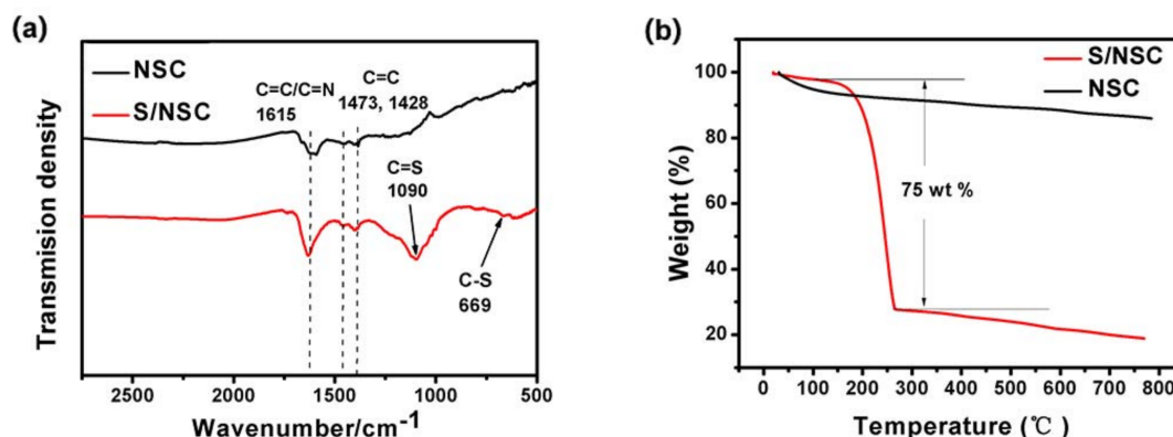
Figure 2. (a) Fourier transform infrared spectroscopy (FTIR) spectra of NSC and S/NSC composites; (b) thermogravimetric curve of NSC and S/NSC composites.
