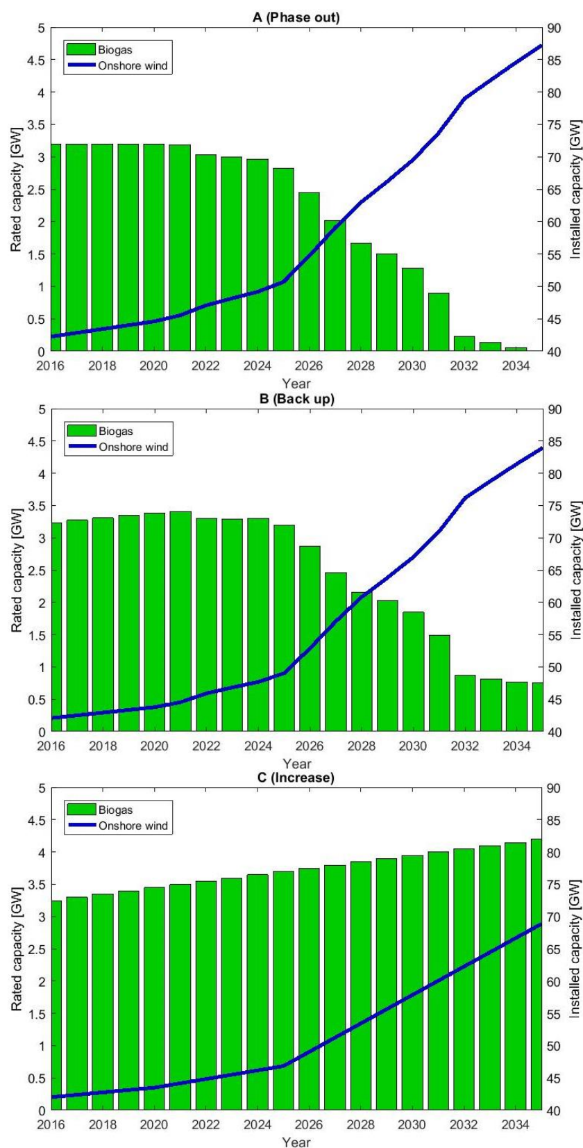
Figure 1. Installed capacities of onshore wind and rated capacities of biogas plants varying the biogas extension paths: biogas phase out (A); biogas back up (B); and biogas increase (C).
