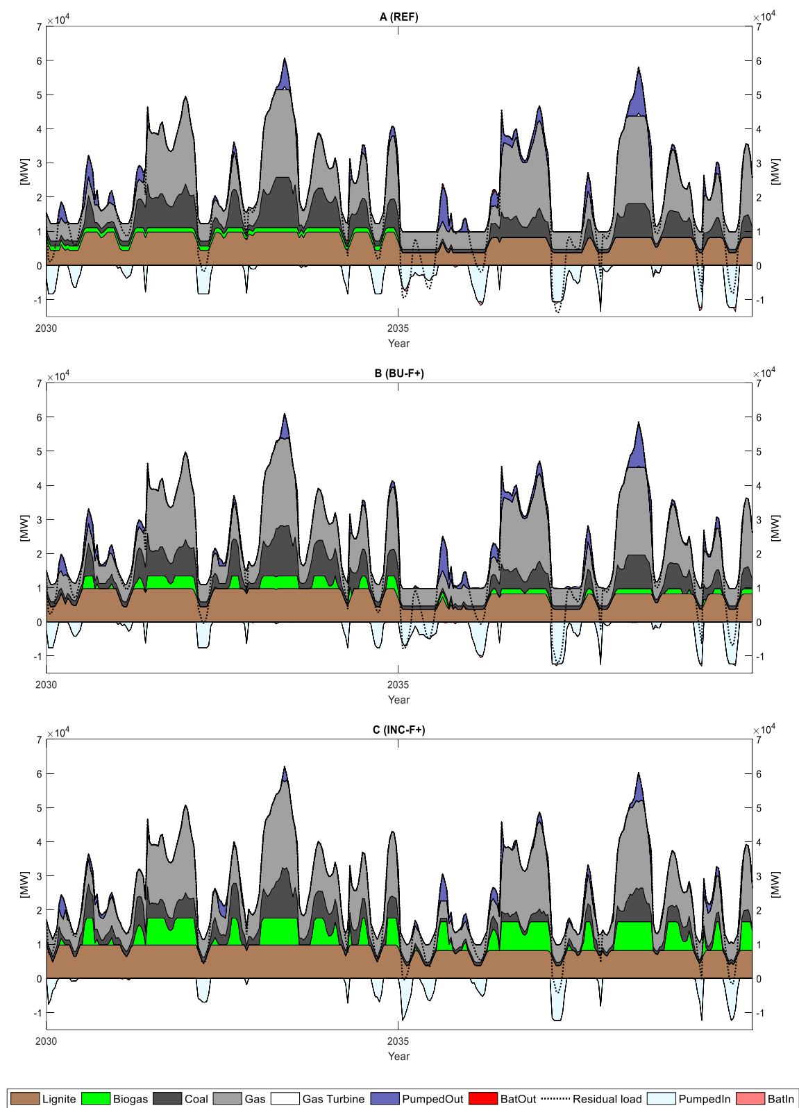
Figure 3. Residual load, biogas, and conventional electricity generation, as well as the operation of the storage technologies in the years 2030 and 2035 in the scenarios REF (A); BU-F+ (B) and INC-F+ (C). PumpedOut: discharged electricity from pumped-storage plants. BatOut: discharged electricity from Li-ion batteries. PumpedIn: charged electricity in pumped-storage plants. BatIn: charged electricity in Li-ion batteries.
