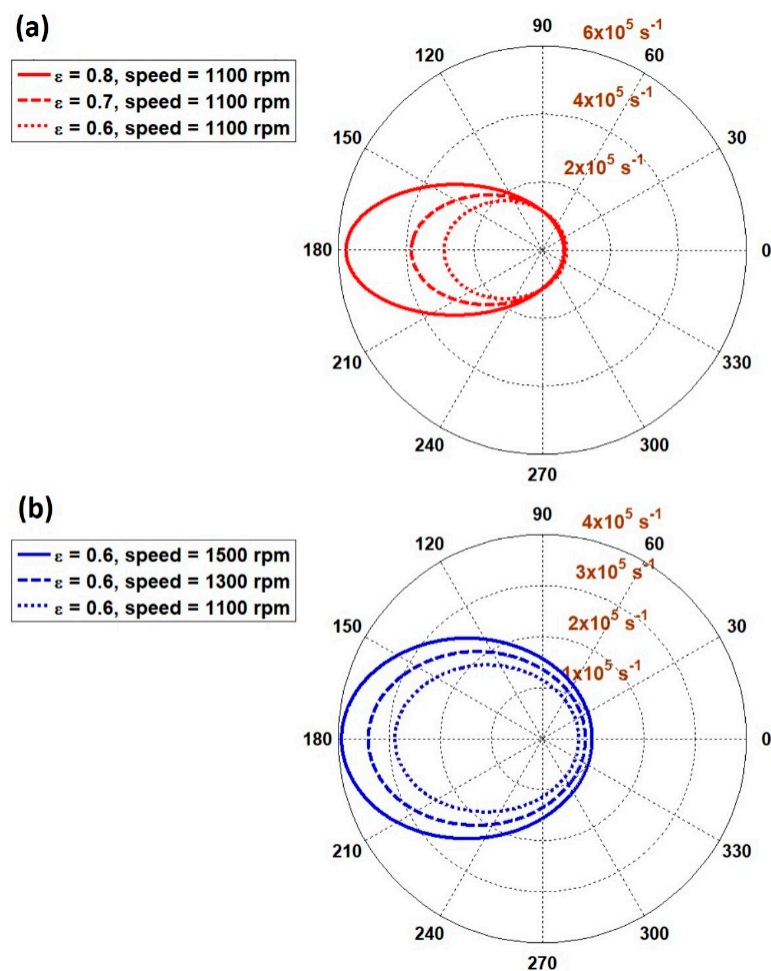
Figure 5. Variation in shear rate along the circumference of the bearing for varying: (a) loads; (b) speeds.
