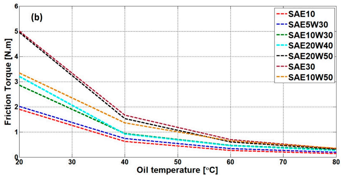
Figure 9. Hydrodynamic frictional torque in a (a) textured journal surface—bearing interface; (b) untextured journal bearing during the warm-up period of an IC engine.
