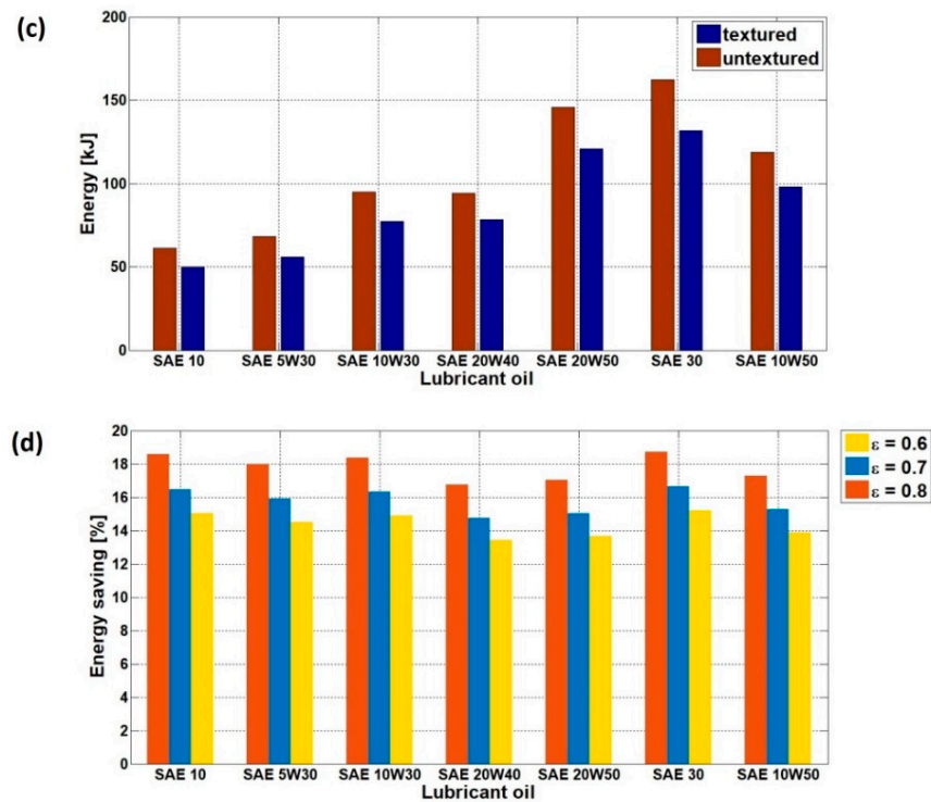
Figure 15. Comparison of fuel energy consumption during engine warm-up period of textured and untextured bearing surfaces at varying loads: (a) \epsilon = 0.6 ; (b) \epsilon = 0.7 ; (c) \epsilon = 0.8 ; (d) percentage of energy saving produced by the surface textures.
