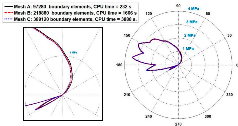
Figure 8. Hydrodynamic pressure variation for varying mesh sizes; mesh-dependency test. The left side of the figure presents a magnified view for a better appreciation of the difference shown in the right side of the figure.
