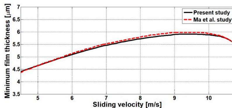
Figure 7. Validation of the mathematical model used in this study.
