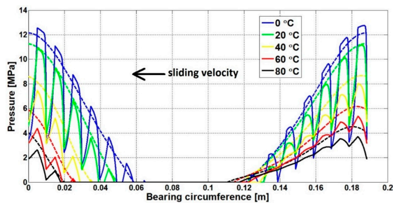
Figure 13. Hydrodynamic pressure and cavitation length variations for textured and untextured plain bearings at the crankshaft of an engine running at 1100 rpm in the warm-up period from 0 °C to 80 °C.
