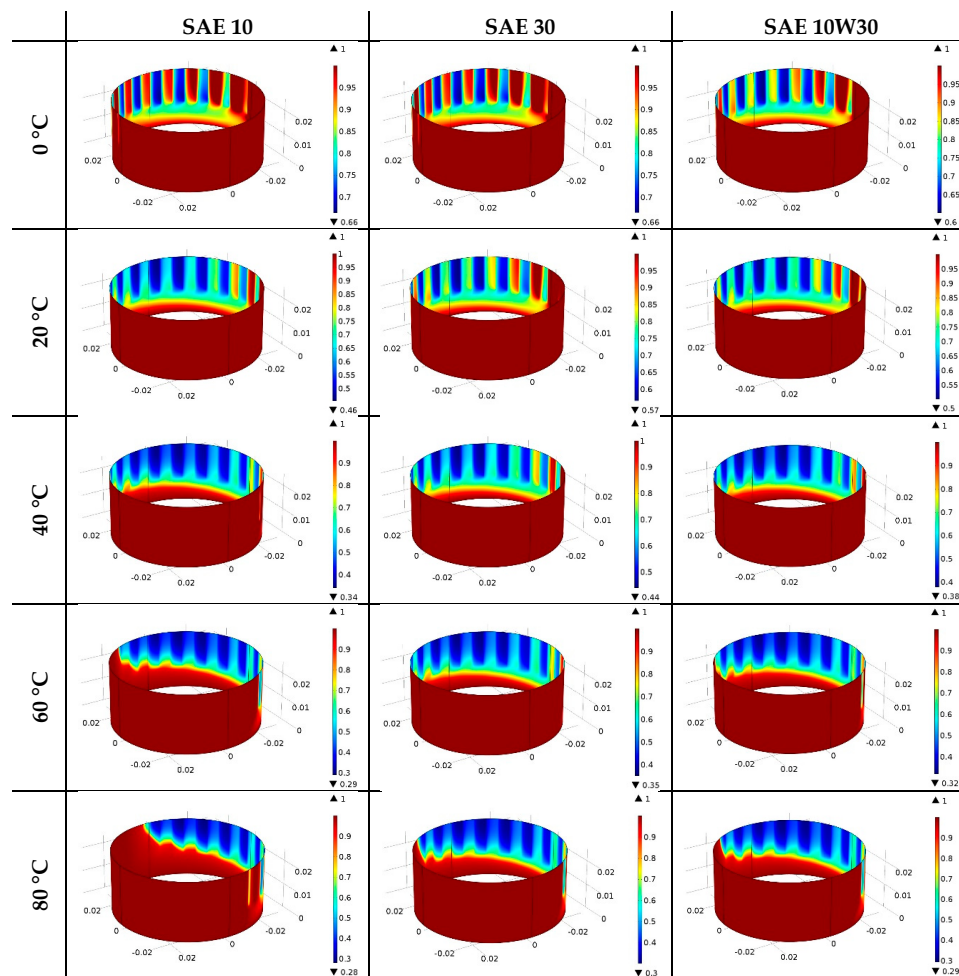
Figure 14. Fractional film content for monograde and multigrade oils at increasing temperatures during engine warm-up.
