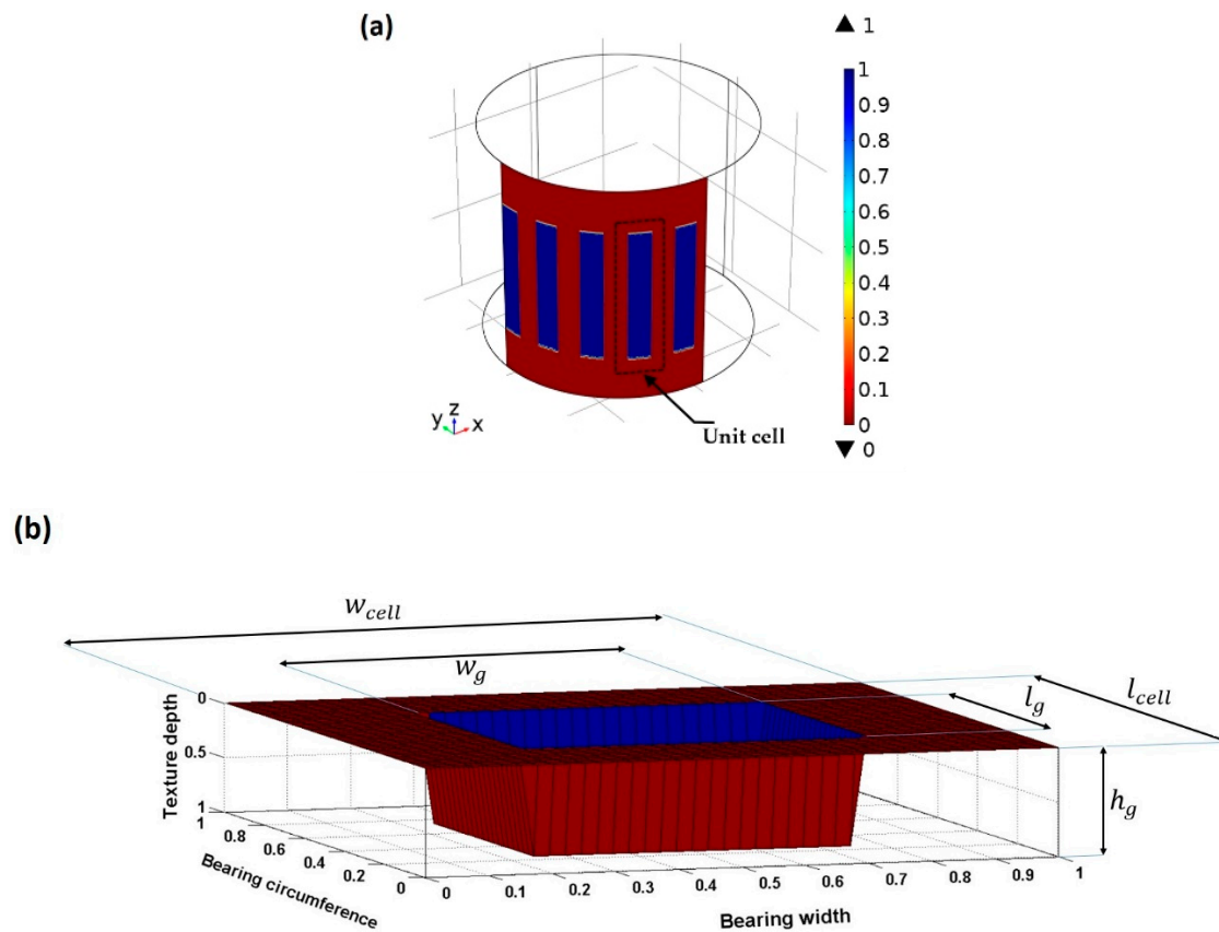
Figure 6. Geometric parameters of a texture in a cell over the journal surface: (a) unit cell representation of the journal surface with dimensionless texture depth; (b) parameter representation in a magnified view.
