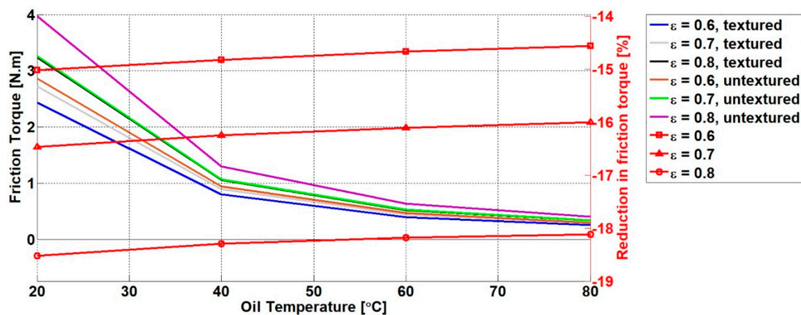
Figure 11. Friction and reduction in the friction for textured and untextured journal bearings at varying loads during the warm-up process of an IC engine.
