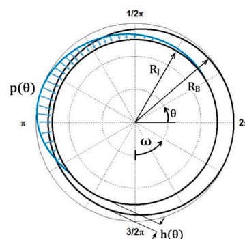
Figure 1. A journal bearing schematic illustration.
