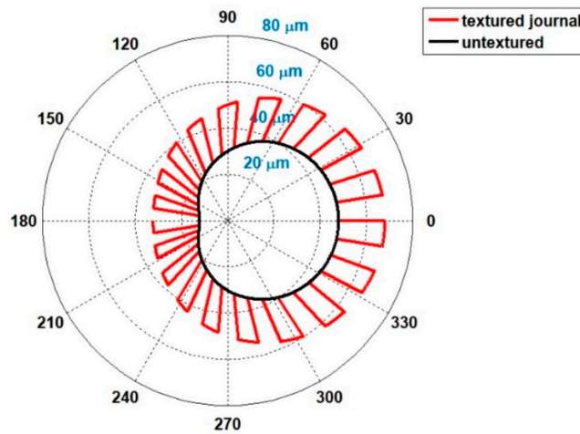
Figure 3. Lubricating oil film thickness at mid-plane of the textured and untextured journal surfaces.
