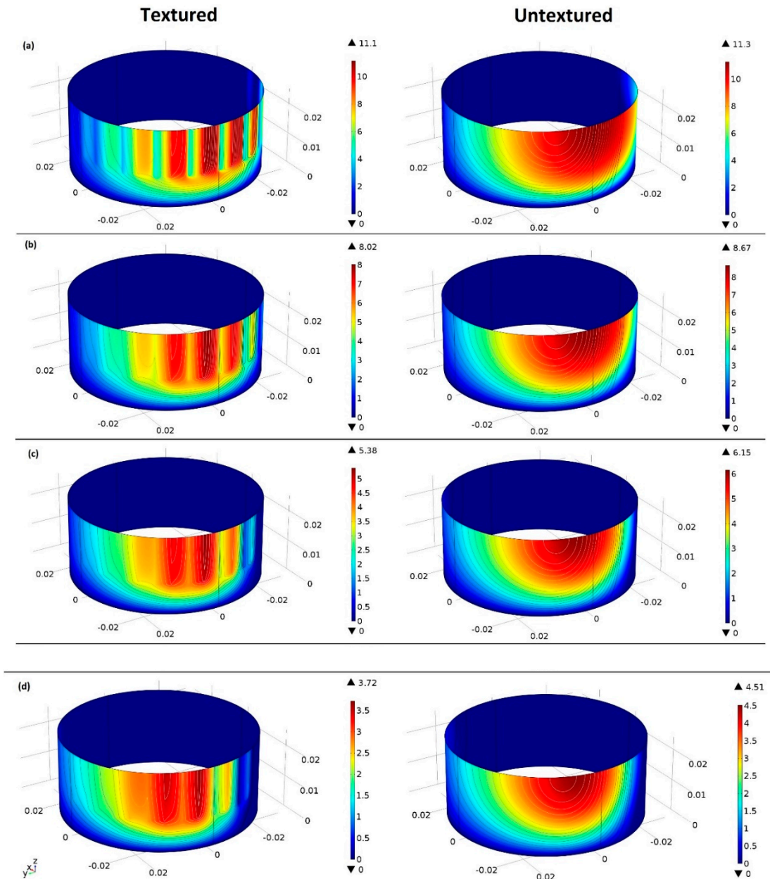
Figure 12. Hydrodynamic pressure (MPa) generation on textured journal bearing compared with the untextured journal bearing at: (a) 20 °C; (b) 40 °C; (c) 60 °C; (d) 80 °C.
