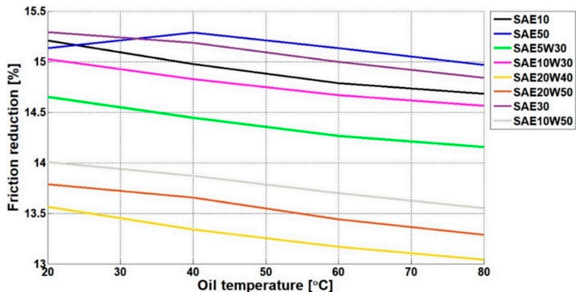
Figure 10. Surface texture-based friction reduction for the journal-bearing interface at varying temperatures of the IC engine for eight different multi- and monograde engine oils.
