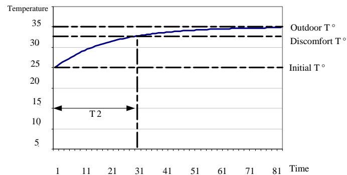
Figure 7. Typical cooling load off cycle during T2 time till discomfort level.
