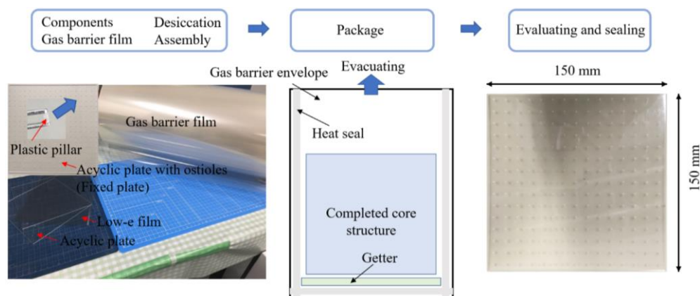
Figure 8. Manufacturing flow of the VIP specimens.
