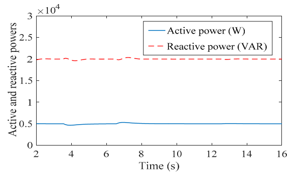
Figure 10. Active and reactive powers of DG.
