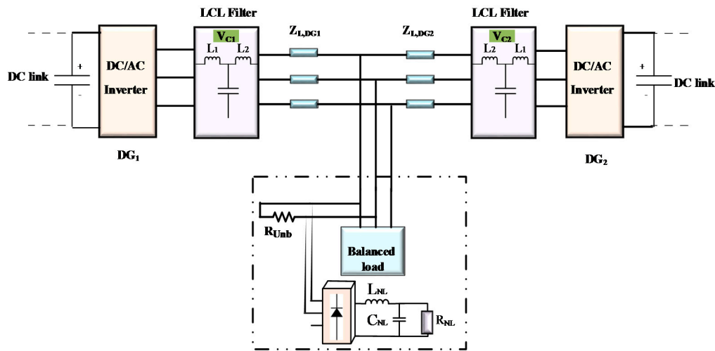
Figure 15. Islanded MG with two DG units.
