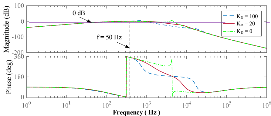
Figure 5. Bode diagram of G_{PSCV} .
