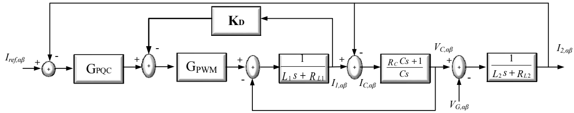
Figure 4. FNS&H current-controller diagram.
