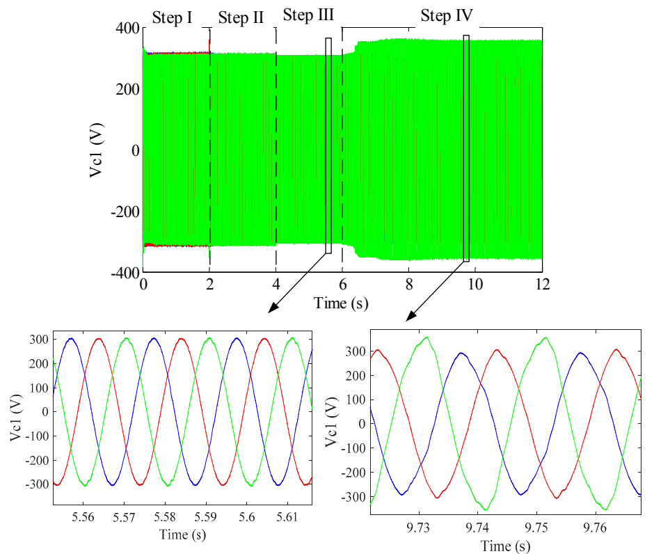
Figure 18. V_{C1} in Step III ( V_C compensation) and Step IV (without compensation) for islanded MG.
