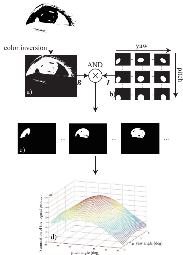
Figure 12. Algorithm for iris tracking using the 3D eye model. An inverted binary image of an eye (a) and the simulated images of the iris area (b) are used to compute the logical product of these image (c). In addition, the iris area is detected when the maximum value is found in the summed values of the logical product (d).
