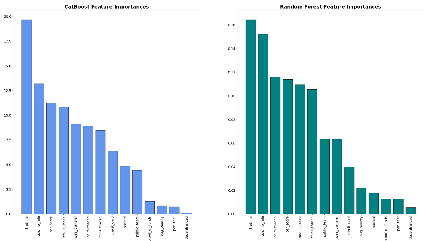
Figure 2. Feature Importance for the Two Best ML Models (CatBoost and Random Forest).
