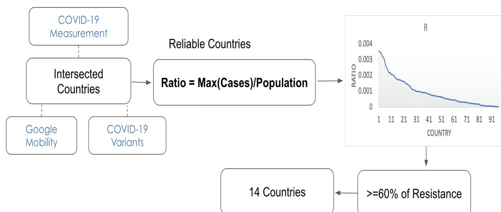
Figure 1. Flowchart of the country selection process based on the largest ratio of detected cases to the population size. Countries that exceed this threshold are included in our dataset if 60% of the population or more have acquired some form of resistance (via vaccination or prior infection) by July 2021.
