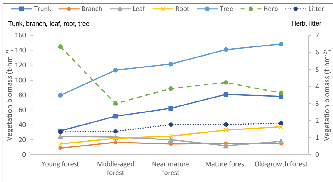
Figure S1. The biomass in different forest age groups.
