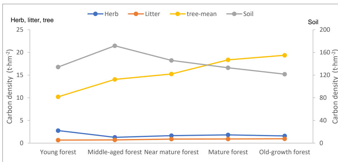
Figure S2. The carbon density of forest layers in different forest age groups.
