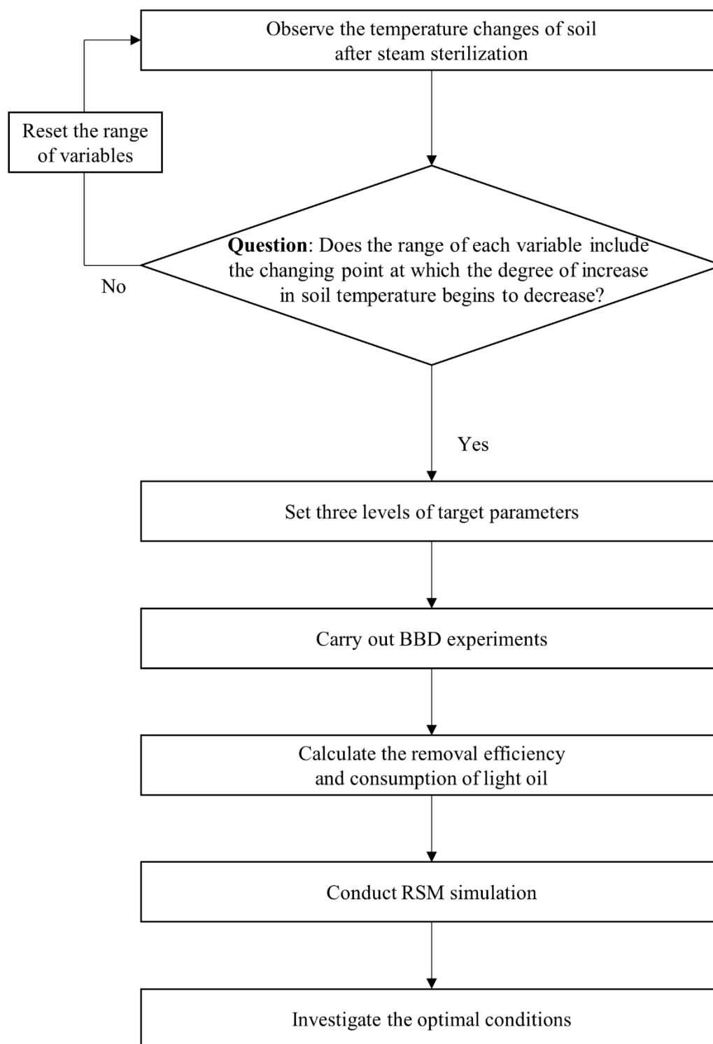
Figure S1. Flow chart of the optimization design.
