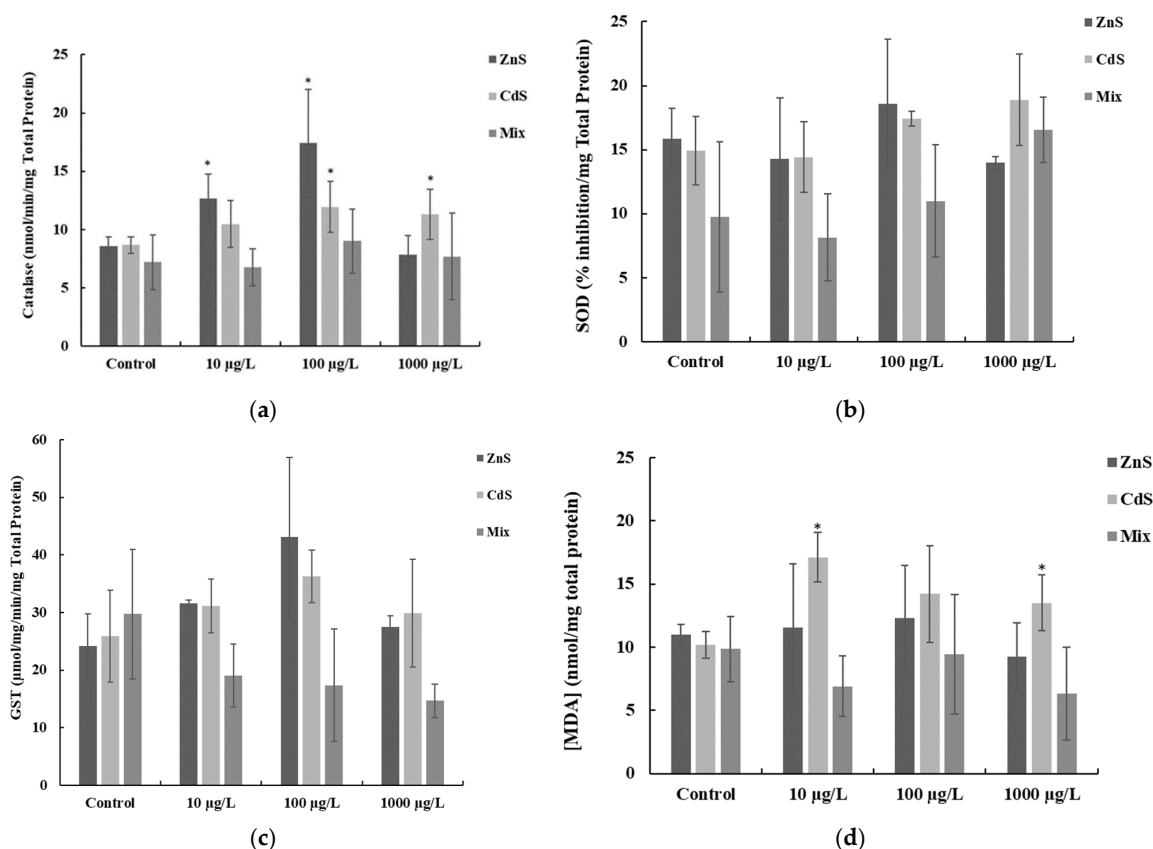
Figure 2. Antioxidant enzymes activities (mean ± SD): (a) CAT, (b) SOD (c) GST; and (d) Lipid peroxidation (MDA content) in zebrafish exposed to different concentrations of QDs, alone and combined (Mix). Asterisk means significant differences ( p < 0.05 ) in comparison to the respective controls.
