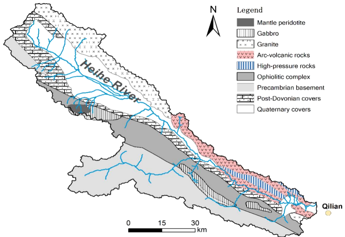
Figure S1. Geological map of the headwater regions of Heihe River Basin.
