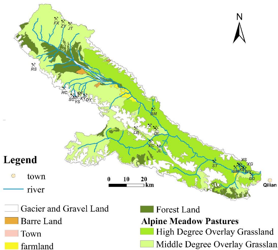
Figure S2. The Land Use Coverage of the headwater region of the Heihe River Basin.
