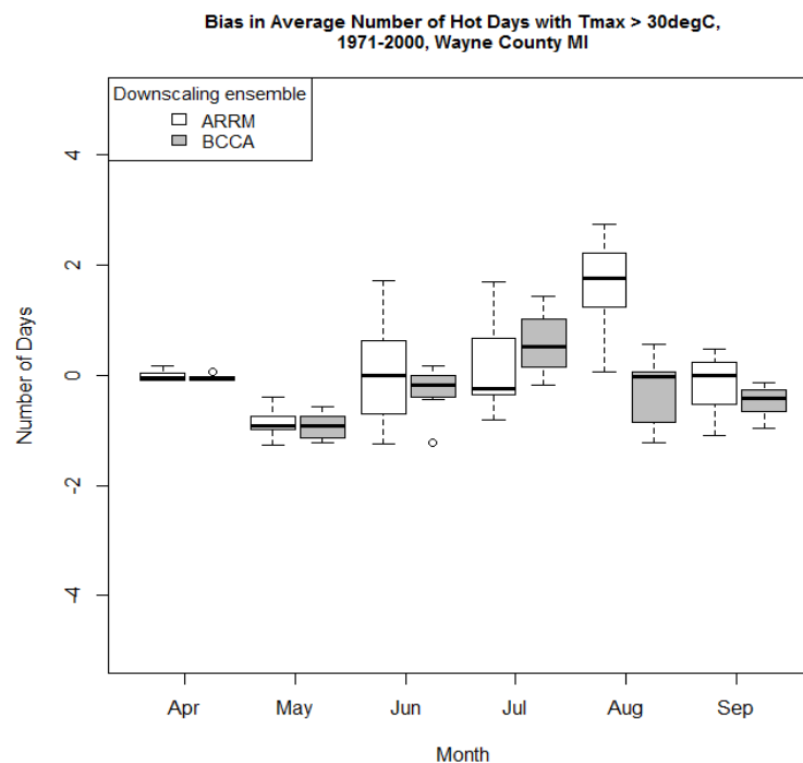
Figure 3. Absolute bias relative to Maurer02v2_1/8 observational dataset of the period mean HD30 in (a) Washington DC area and (b) Wayne County MI for 1971–2000 as represented by the ARRM and BCCA ensembles at 1/8° latitude resolution. Heavy line within each box plot represents the median.
