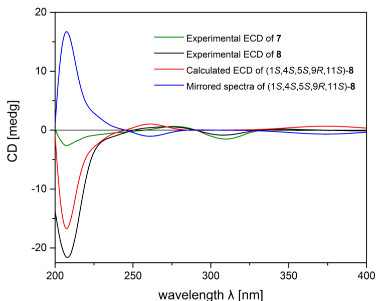
Figure 8. Experimental ECD spectra of 7 (green), 8 (black), calculated ECD spectrum of (1S,4S,5S,9R,11S)-8 (red), and mirrored spectra of (1S,4S,5S,9R,11S)-8 (blue).
