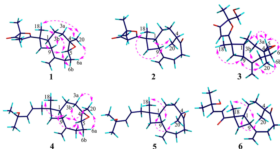
Figure 3. Key NOESY correlations of compounds 1–6.
