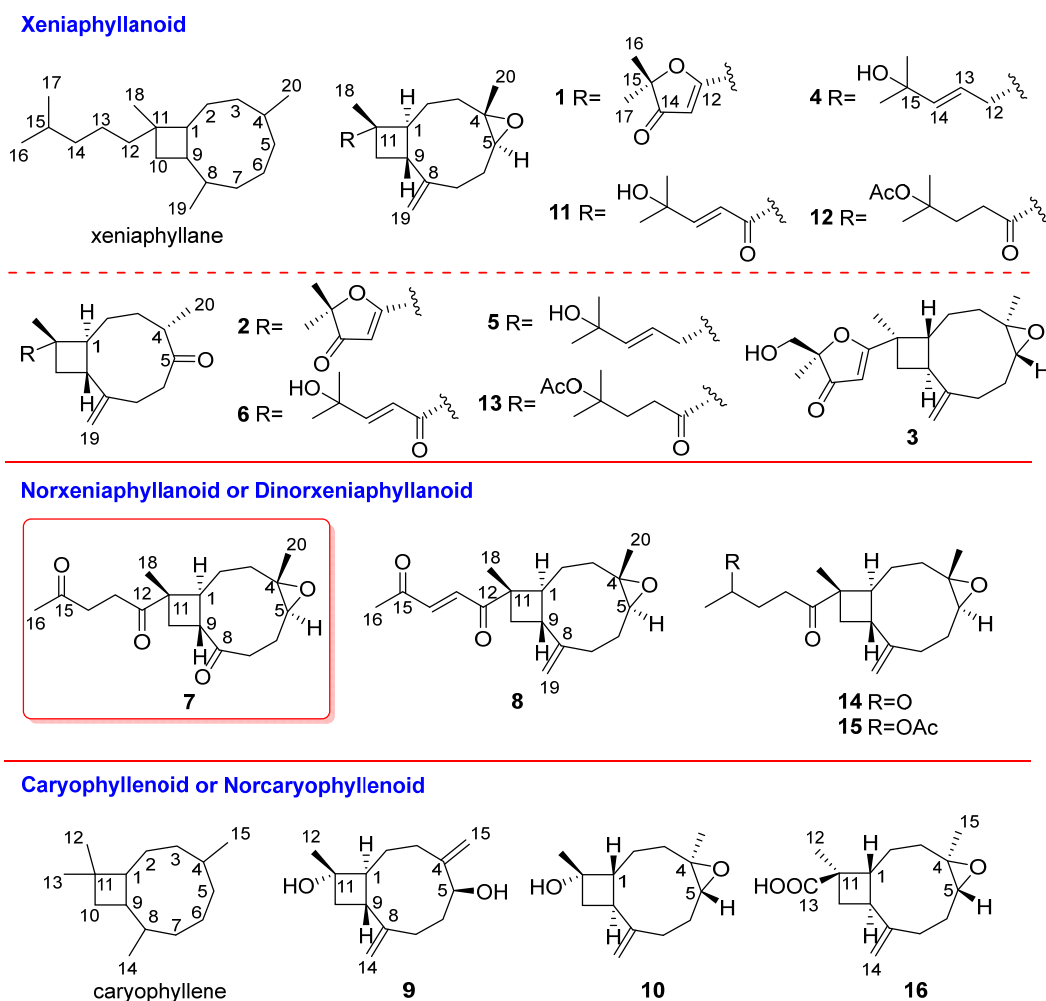
Figure 1. Structures of compounds 1–16, xeniaphyllane, and caryophyllene.
