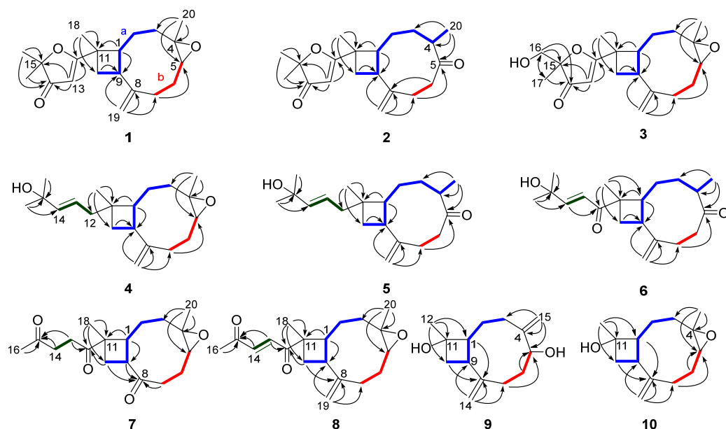
Figure 2. Selected ^1\text{H} – ^1\text{H} COSY (bold lines) and key HMBC (single arrows) correlations of 1–10. Fragments a (blue) and b (red) represent two different spin systems, respectively.
