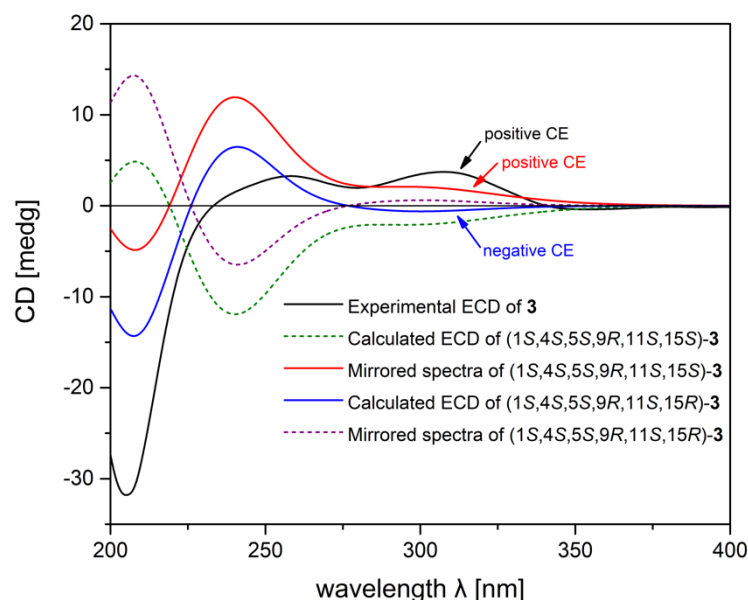
Figure 5. Experimental ECD spectra of 3 (black), calculated ECD spectrum of (1 S ,4 S ,5 S ,9 R ,11 S ,15 S )- 3 (dashed green), mirrored spectra of (1 S ,4 S ,5 S ,9 R ,11 S ,15 S )- 3 (red), calculated ECD spectrum of (1 S ,4 S ,5 S ,9 R ,11 S ,15 R )- 3 (blue), and mirrored spectra of (1 S ,4 S ,5 S ,9 R ,11 S ,15 R )- 3 (dashed purple).
