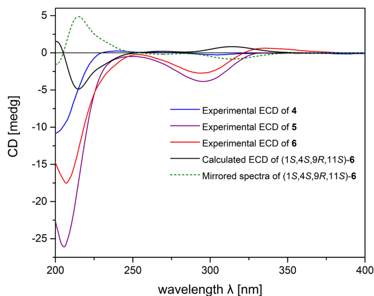
Figure 6. Experimental ECD spectra of 4 (blue), 5 (purple), 6 (red), calculated ECD spectrum of (1S,4S,9R,11S) - 6 (black), and mirrored spectra of (1S,4S,9R,11S) - 6 (dashed green).
