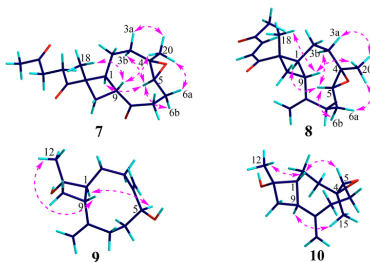
Figure 7. Key NOESY correlations of compounds 7–10.
