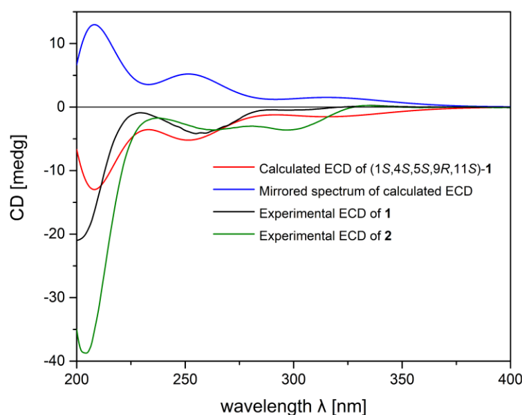
Figure 4. Experimental ECD spectrum of 1 (black) and 2 (green); calculated ECD spectrum of (1 S ,4 S ,5 S ,9 R ,11 S )- 1 (red) and its enantiomer (blue).
