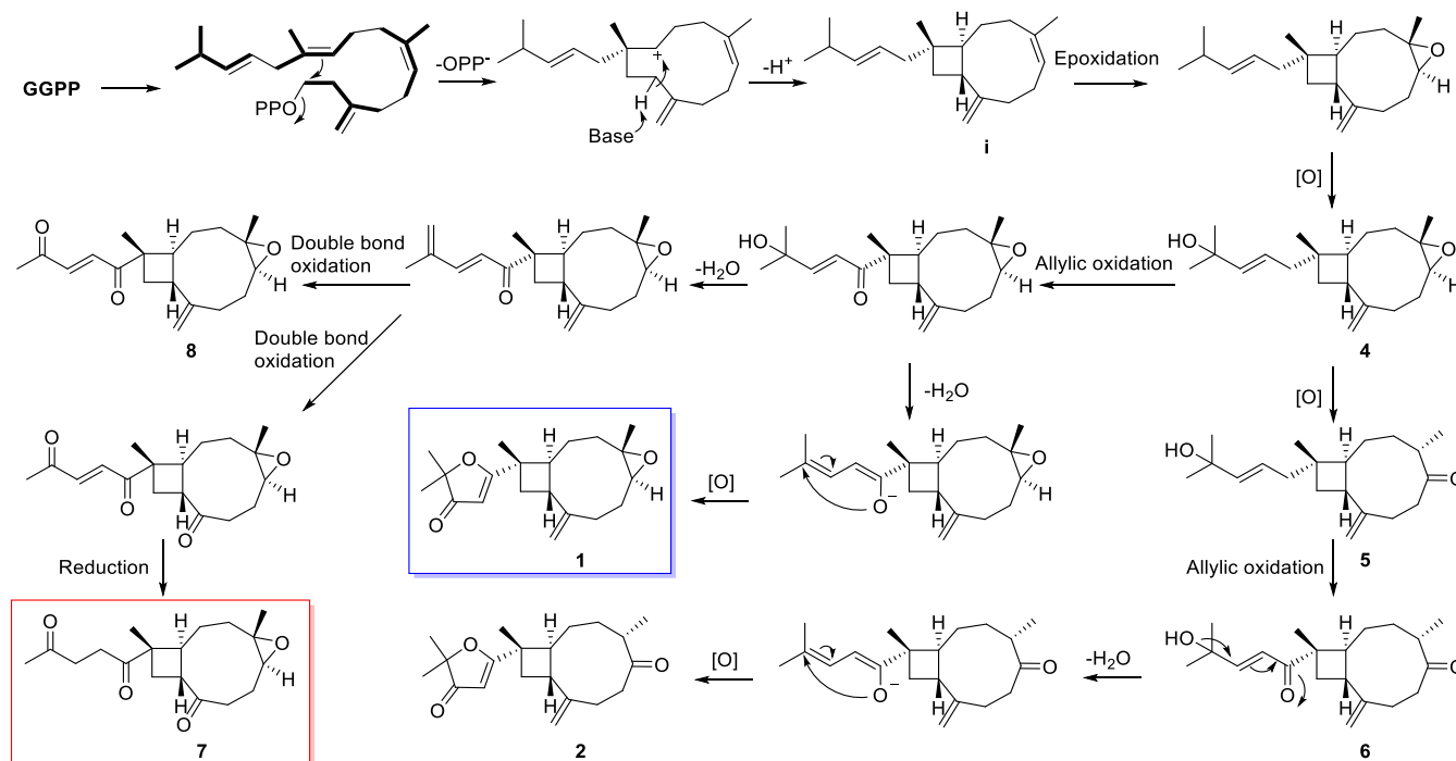
Scheme 1. Plausible biosynthetic connection between compounds 1–9 (OPP: diphosphate).
