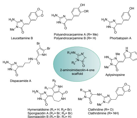
Figure 1. Structures of a selection of marine natural products sharing the 2-aminoimidazol-4-one scaffold.
