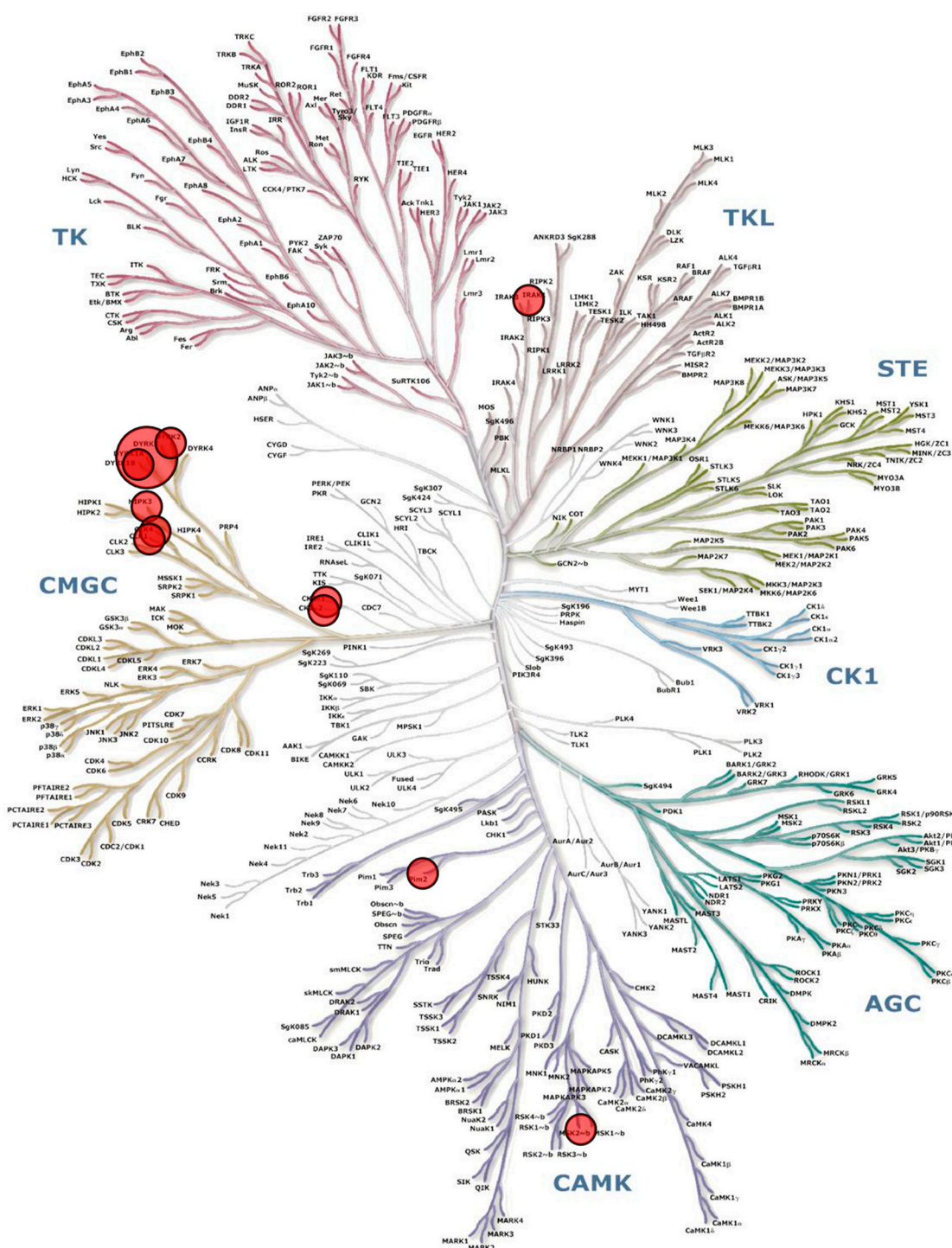
Figure 2. TREEspot™ kinase interaction map of polyandrocarpine A with 442 human kinases (DiscoverX KinomeScan®, San Diego, CA, USA). Polyandrocarpine A was tested at a 1 \mu M final concentration in the kinase interaction panel. A semi-quantitative scoring of this primary screen was estimated. This score relates to a probability of a hit rather than strict affinity. Scores >10, between 1–10 and <1 indicate that the probability of being a false positive is <20%, <10%, <5%, respectively. Results are presented in Table 2 and here as a TREEspot™ kinase interaction maps. Circles indicate the major hits and their size is proportional to the scores. All 442 values are provided in the Supplementary Table S4.
