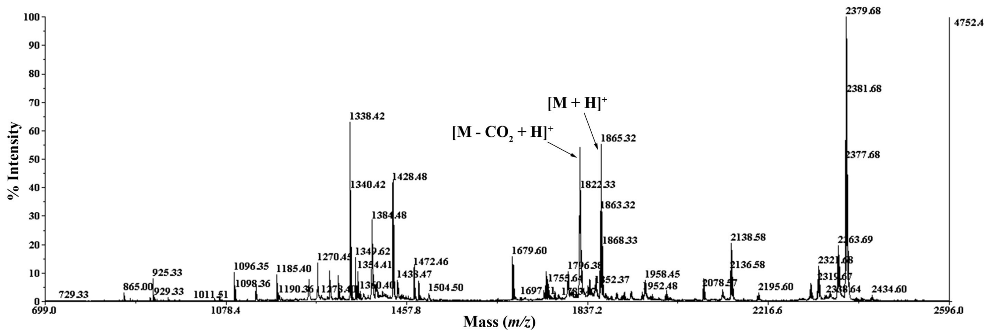
Figure S1. The MALDI-TOF spectra of the fraction “3.2” highlighted in black in Figure 1B.
