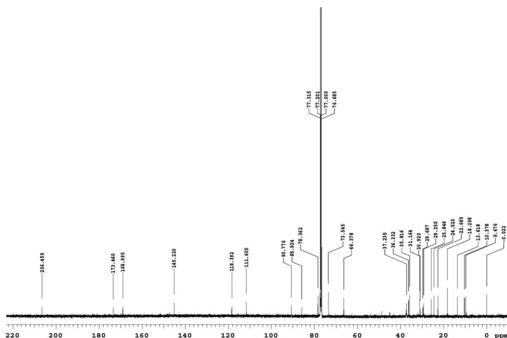
Figure S15. ^{13}\text{C} NMR spectrum of 5 in \text{CDCl}_3 .
