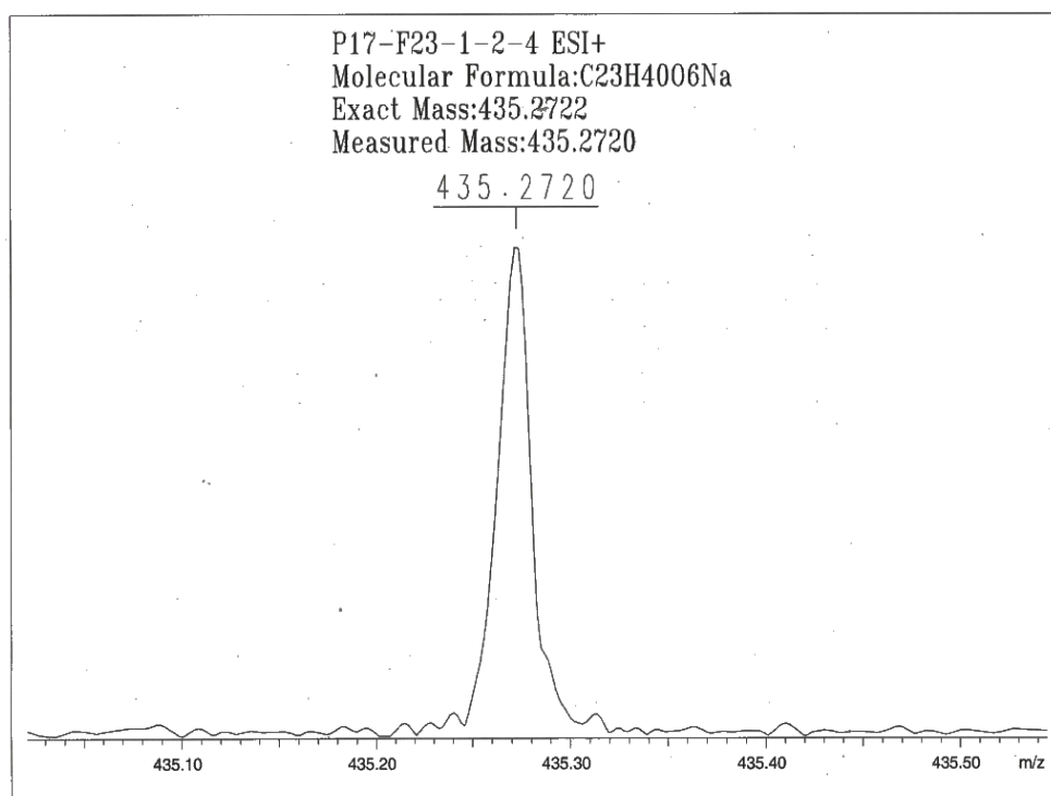
Figure S7. HREIMS spectrum of 3.
