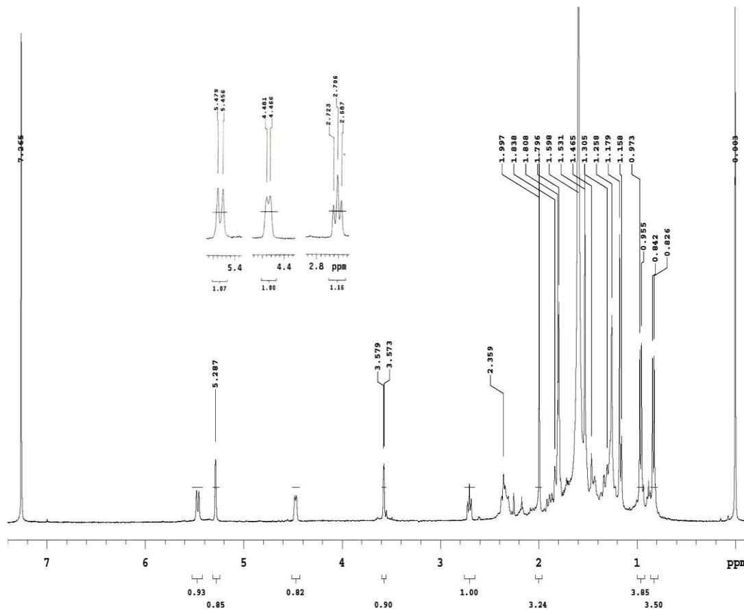
Figure S11. 1 H NMR spectrum of 4 in CDCl 3 .
