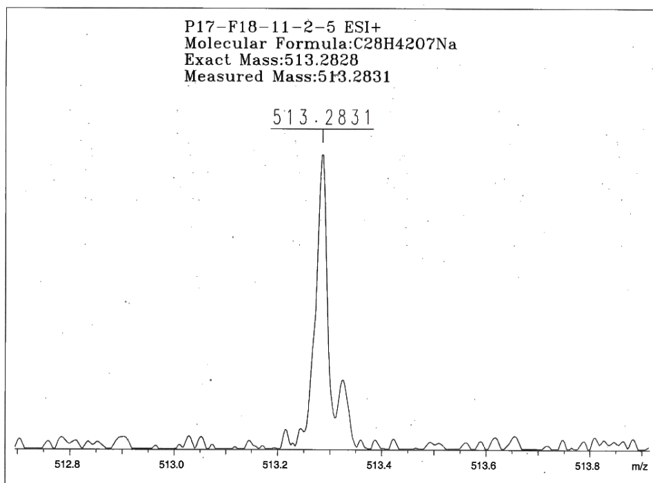
Figure S13. HREIMS spectrum of 5 .
