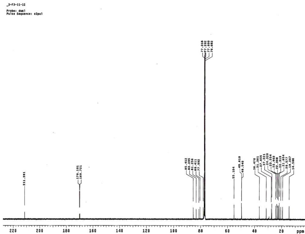
Figure S3. ^{13}\text{C} NMR spectrum of 1 in \text{CDCl}_3 .
