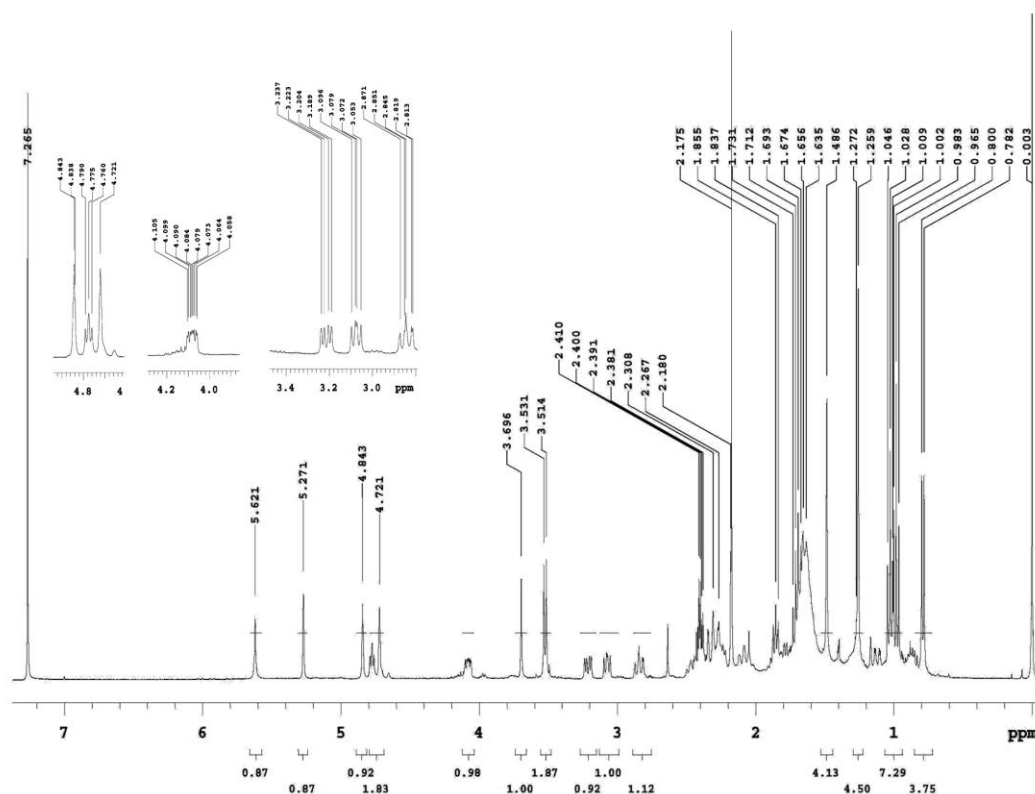
Figure S14. ^1\text{H} NMR spectrum of 5 in \text{CDCl}_3 .
