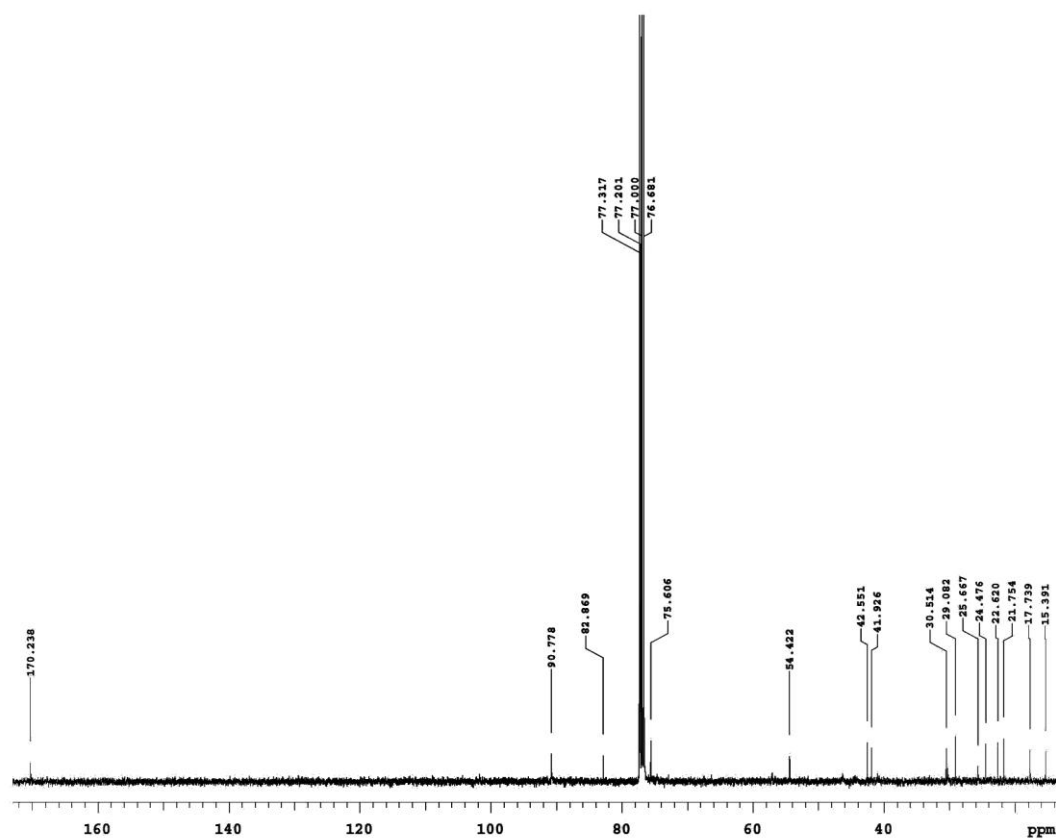
Figure S9. ^{13}\text{C} NMR spectrum of 3 in \text{CDCl}_3 .
