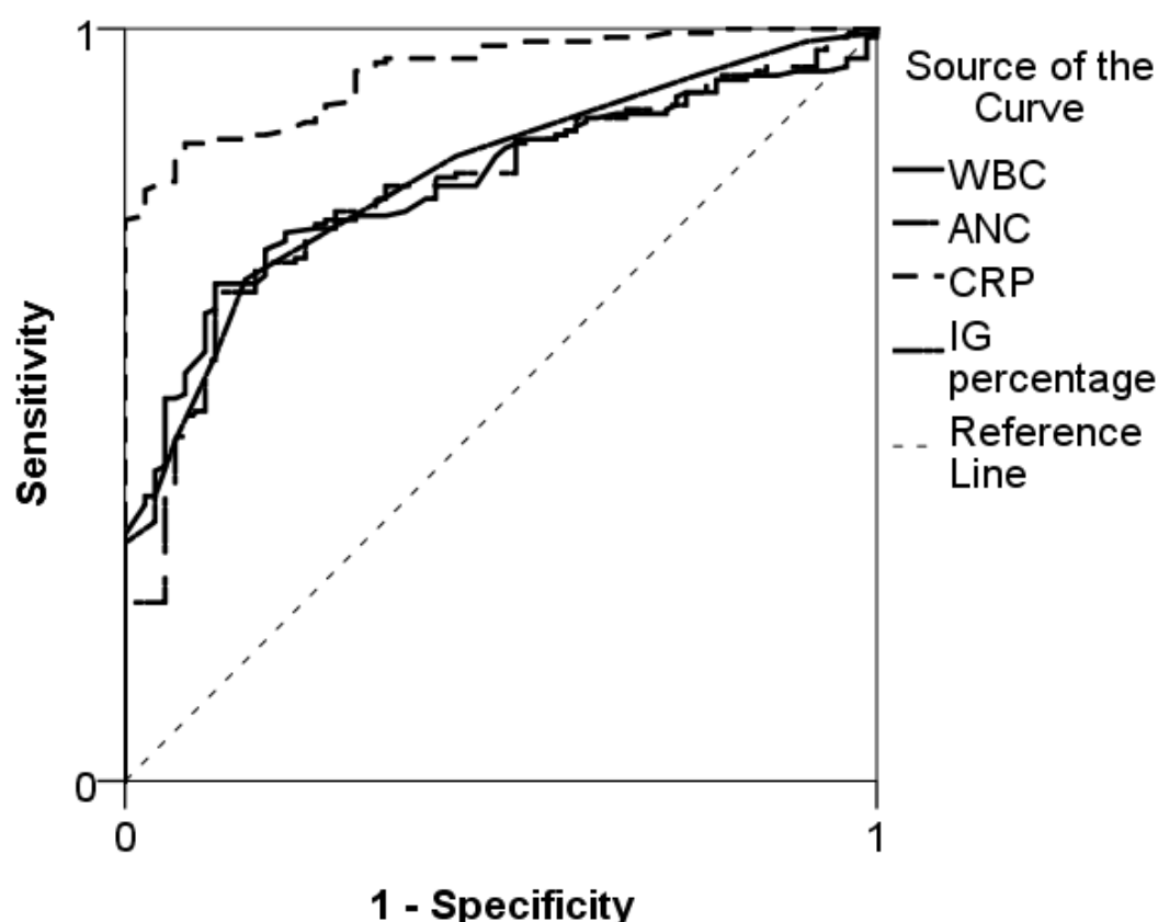
Figure 1. Receiver operating curves for immature granulocyte (IG) percentage, white blood count (WBC), absolute neutrophil count (ANC), and C-reactive protein (CRP) in predicting serious bacterial infections in children.
