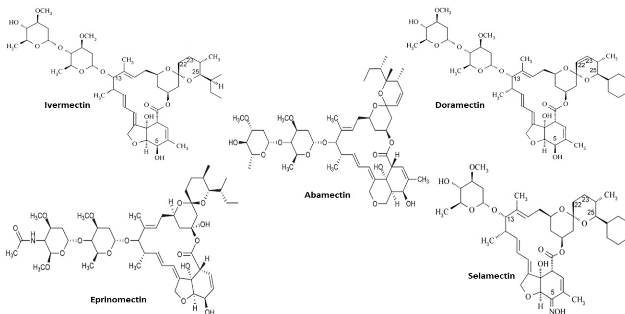
Figure 2. Chemical structure of various avermectins.
