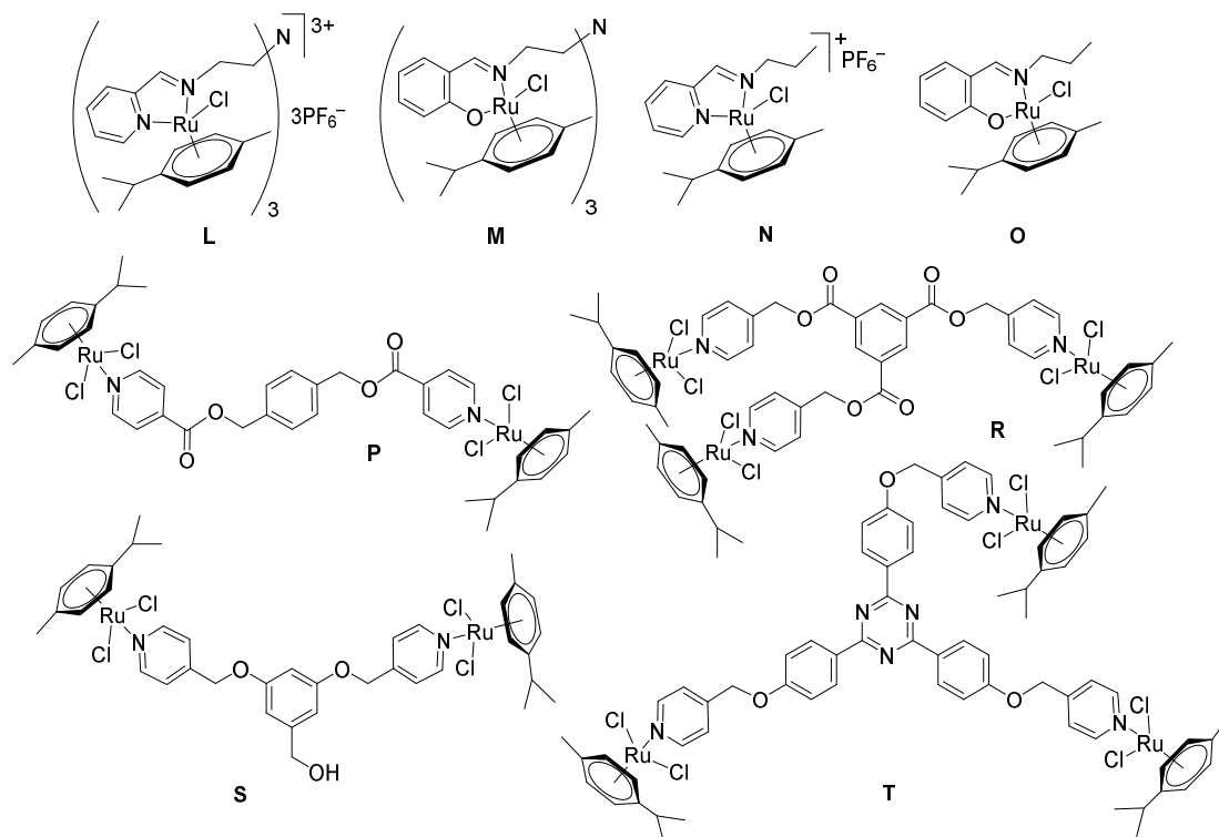
Figure 3. Structure of star-shape trinuclear L and M , and of the mononuclear N and O Ru(II)- p -cymene complexes with Schiff-base ligands; structure of di- ( P and R ) and trinuclear ( S and T ) ruthenium(II)- p -cymene complexes with polypyridyl ester and ether ligands.
