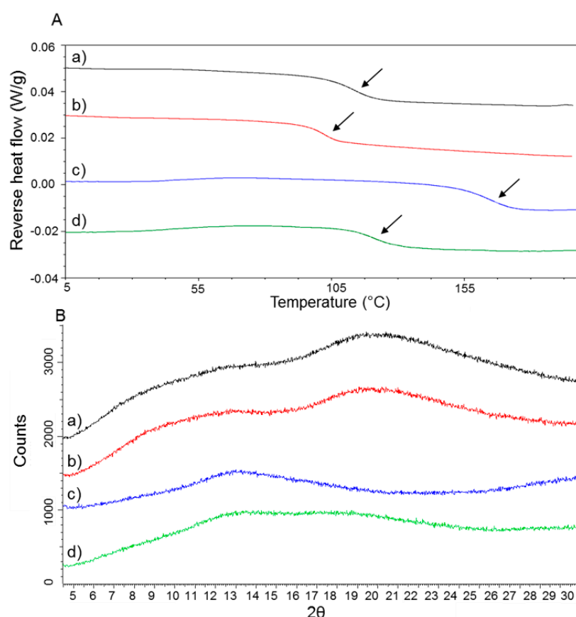
Figure 4. Reverse heat flow signals (A) and X-ray powder diffraction (XRPD) patterns (B) of 40:60 ( w/w ) CDP146 SDSDs (20 mg) made with HPMCP HP50 (a), HPMCAS-LF (b), Eudragit L100 (c) and Eudragit L100-55 (d).
