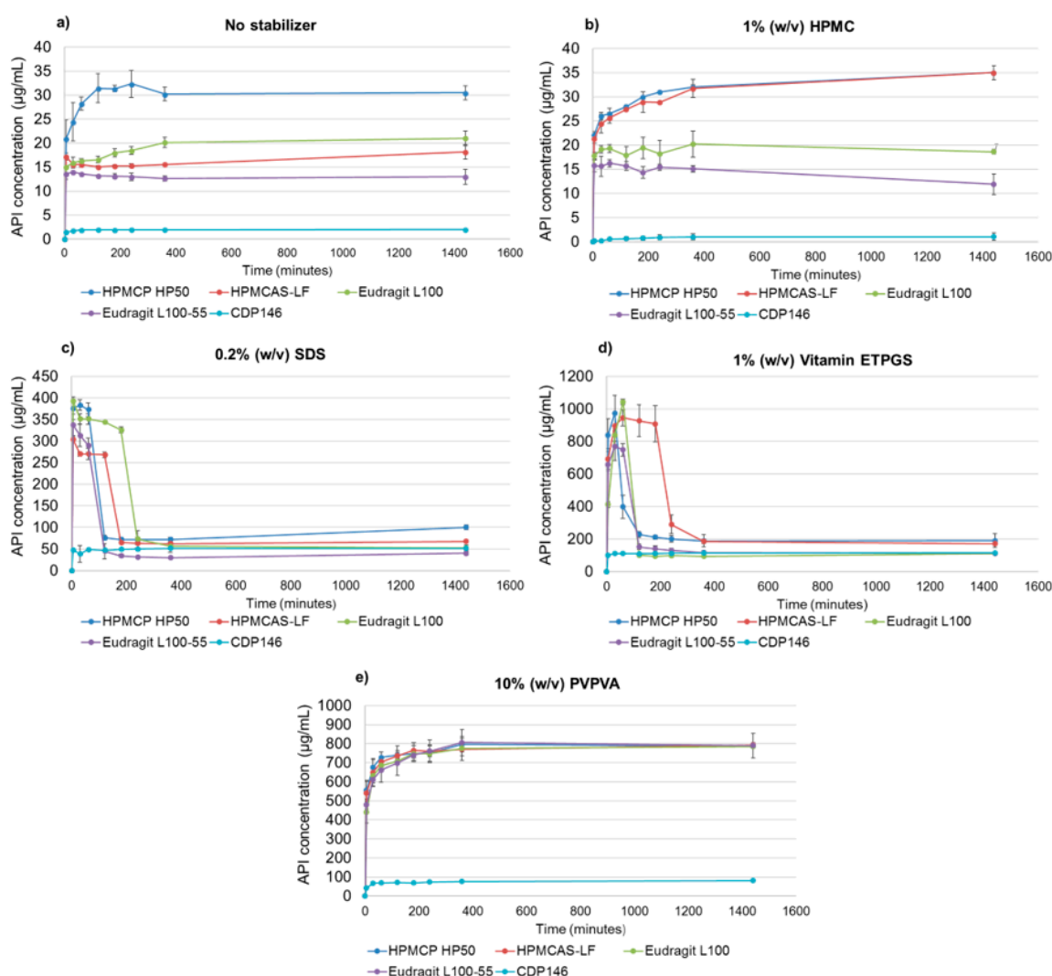
Figure 6. Dissolution profiles of 40:60 ( w/w ) CDP146 SDSDs (100 mg) and pure crystalline API in 50 mM phosphate buffer (pH 6.5) without stabilizer (a) or with 1% ( w/v ) HPMC (b), 0.2% ( w/v ) SDS (c), 1% ( w/v ) Vitamin ETPGS (d) and 10% ( w/v ) PVPVA (e) at an API concentration of 1 mg/mL.
