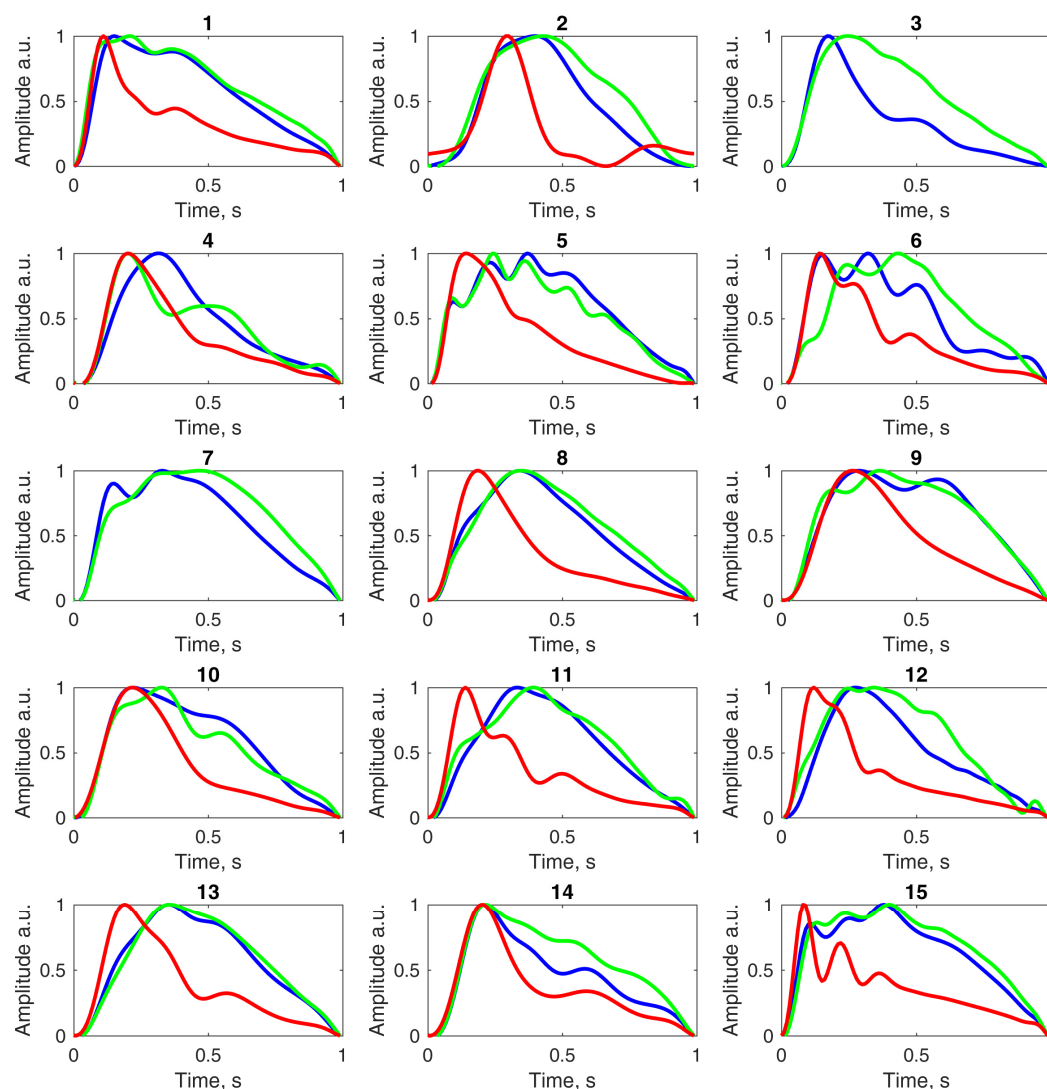
Figure 4. Averaged and normalized pulse waveforms of invasive ICP (blue), non-invasive ICP obtained with the Archimedes O2 device (green), and invasive ABP (red), recorded simultaneously. The number above each signal panel indicates the corresponding ICU patient.
