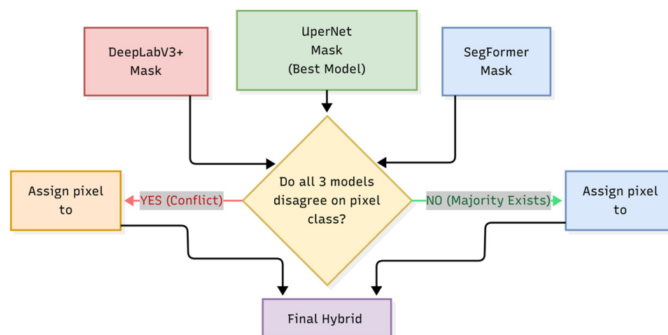
Figure 7. Majority voting and final segmentation map synthesis algorithm.
