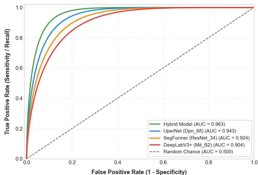
Figure 10. ROC curve of segmentation results.
