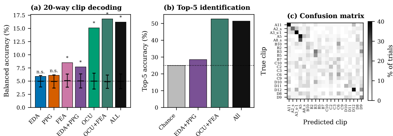
Figure 8. Multimodal decoding of clip identity. (a) Balanced accuracy by feature set; horizontal markers with error bars represent the mean and 95% range of the within-participant permutation null, and the dotted line marks the 5% chance level; *, p < 0.05 against the permutation null; n.s., not significant. (b) Top-5 accuracy against a 25% chance level, marked by the dotted line. (c) Row-normalized confusion matrix of the full multimodal model. EDA, electrodermal activity; PPG, photoplethysmographic pulse; FEA, facial expression analysis; OCU, oculomotor.
