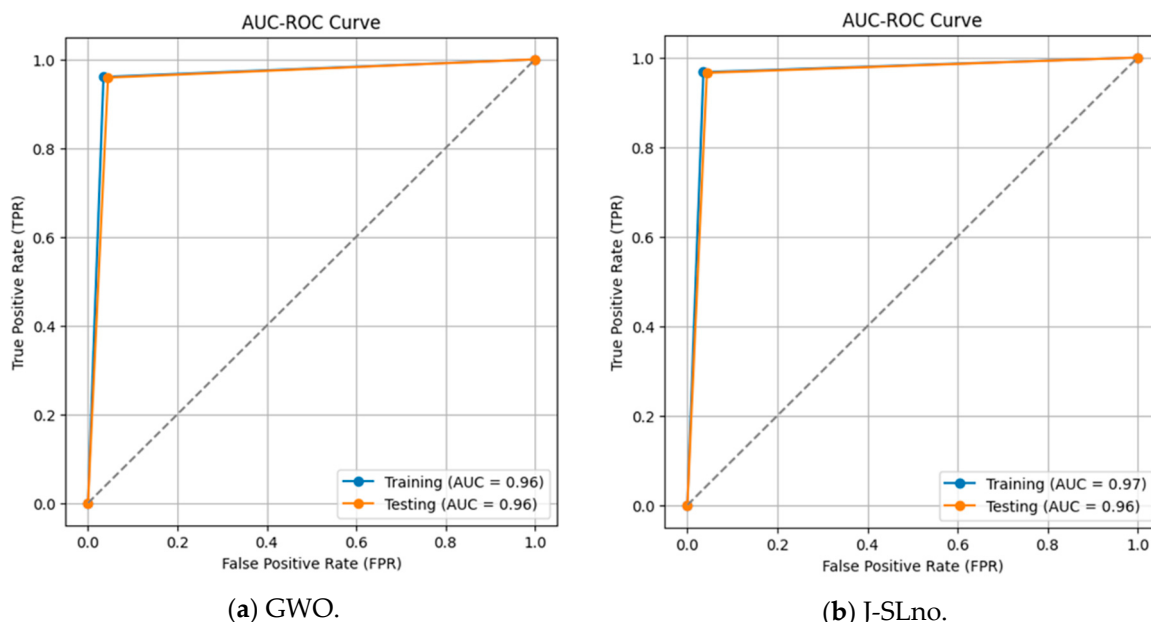
Figure 9. ROC-AUC curve.
