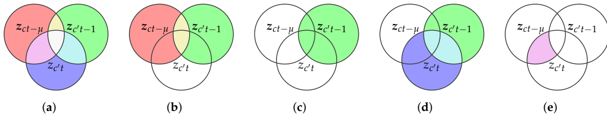
Figure 1. Venn diagrams illustrating the definition of Transfer Entropy from joint and marginal Shannon entropies: Circles correspond to the responding channel present z_{c't} (blue), the Takens-embedded responding's past z_{c't-1} (green), and the Takens-embedded driving's past z_{ct-\mu} (red). The Transfer Entropy identifies the unique predictive information from the driving's past to the responding's present beyond the responding's own history. (a) Joint entropy H_S\{z_{c't}, z_{c't-1}, z_{ct-\mu}\} . (b) Marginal entropy H_S\{z_{c't-1}, z_{ct-\mu}\} . (c) Marginal entropy H_S\{z_{c't-1}\} . (d) Marginal entropy H_S\{z_{c't}, z_{c't-1}\} . (e) Resulting TE(c \rightarrow c') .
