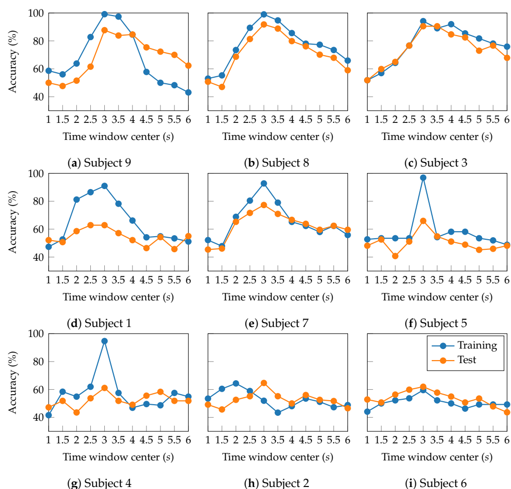
Figure 10. Classification accuracy for each subject across overlapping time windows during the 7-s motor imagery task. A total of 11 time windows were used, each with a 0.5-s overlap. The x-axis represents the center of each time window, and the y-axis shows the classification accuracy (%). This analysis reveals temporal dynamics in classification performance throughout the motor imagery period.
