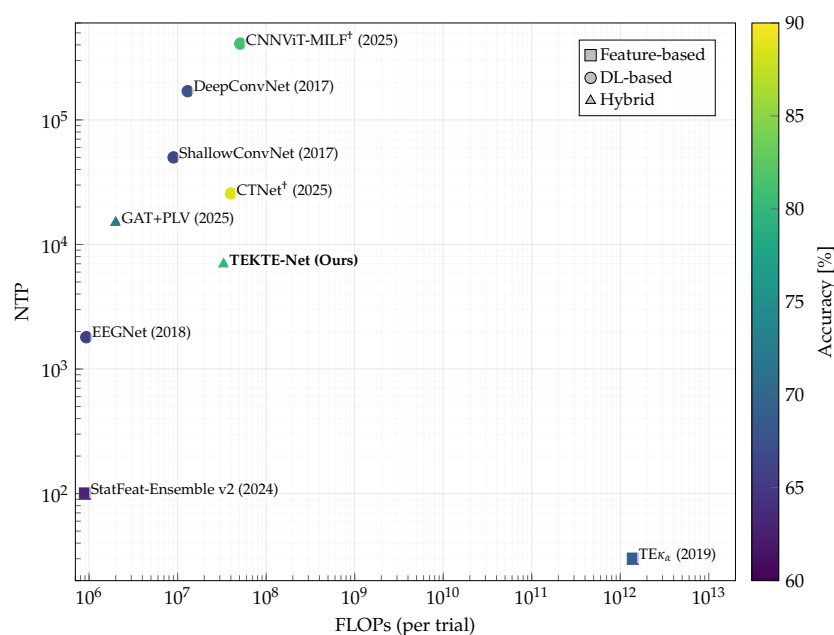
Figure 13. State-of-the-art comparison for binary MI-EEG decoding in terms of Floating Point Operations (FLOPs), number of trainable parameters (NTP), and testing accuracy. † Accuracy reported on the BCI Competition IV-2b testing set (Left vs. Right).
