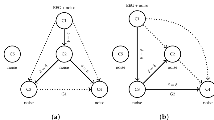
Figure 4. Causal structures of the synthetic benchmarks used for validation. Each configuration consists of one real EEG, three synthetic, and one noise channels. Causal interactions are different between the two structures. (a) G1. (b) G2.
