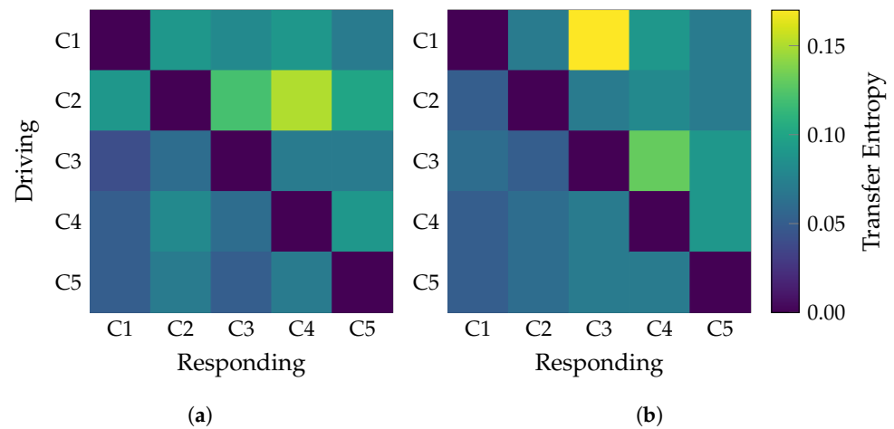
Figure 5. Average TE matrices for the semi-synthetic causal structures G1 and G2. Each matrix captures the dominant directed interactions estimated by the TEKTE-Net. (a) G1-Transfer Entropy Matrix. (b) G2-Transfer Entropy Matrix.
