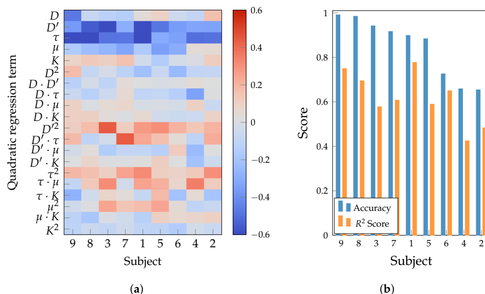
Figure 8. Results of the Bayesian hyperparameter optimization for subjects descending-sorted according their validation accuracy. (a) Quadratic regression coefficients from validation accuracy to hyperparameters. (b) Regression and classification performances for validation data.
