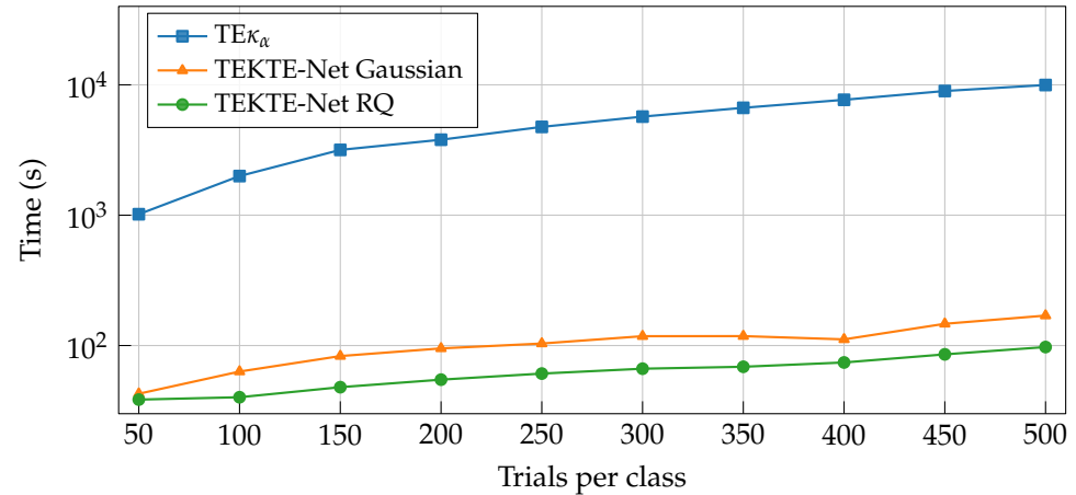
Figure 7. Scalability test for TE\kappa_\alpha and TEKTE-Net: Total training vs. the number of trials per class.
