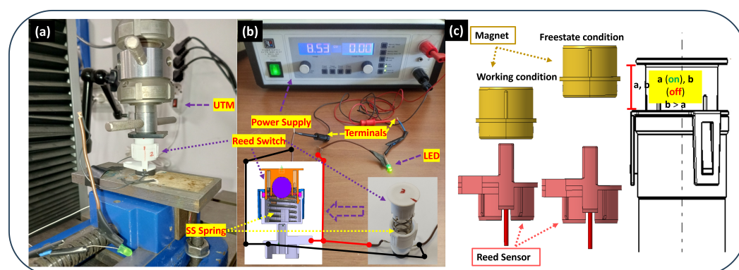
Figure 3. Switching performance of reed sensors with straight terminal spring-integrated prototype testing: (a) precise switching distance measurement using a Universal Testing Machine (UTM), (b) electrical connectivity verification setup showing the power supply and measurement instruments, and (c) schematic diagram of activation and release mechanism of reed sensor.
