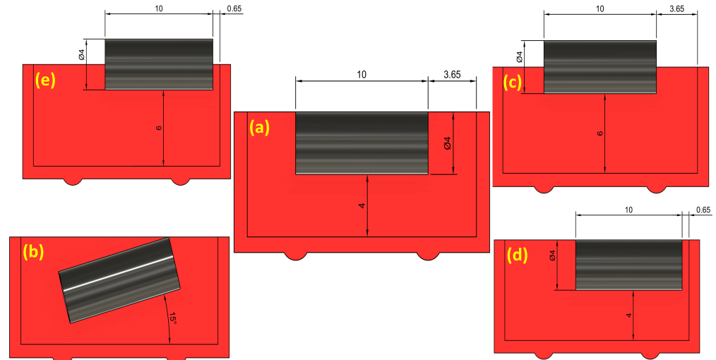
Figure 2. Schematic diagrams of the five tested magnet orientations relative to the reed sensor: (a) center-aligned, (b) center-angled, (c) center upward, (d) right-shift-aligned, (e) right-shift-upward.
