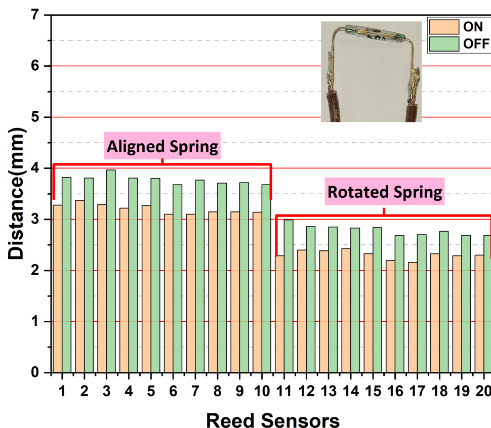
Figure 6. Switching performance of reed sensors with bended terminals, comparing aligned ( 0^\circ ) and rotated ( 90^\circ ) spring orientations.
