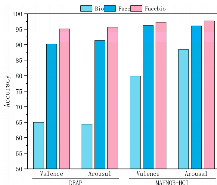
Figure 4. Classification results of ablation experiments (Accuracy).
