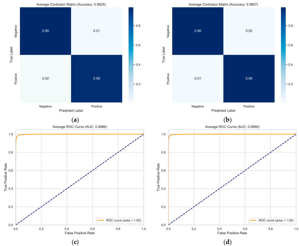
Figure 7. Classification average confusion matrix for the MAHNOB-HCI dataset on the (a) valence and (b) arousal dimensions ROC curves for the (c) valence and (d) arousal dimensions.
