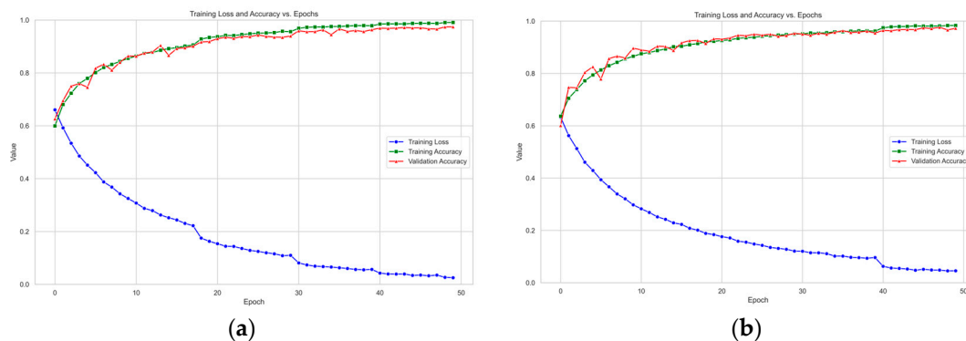
Figure 2. Model performance evaluation curves in the DEAP dataset. Here, (a) represents the Valence dimension curve and (b) represents the Arousal dimension curve.
