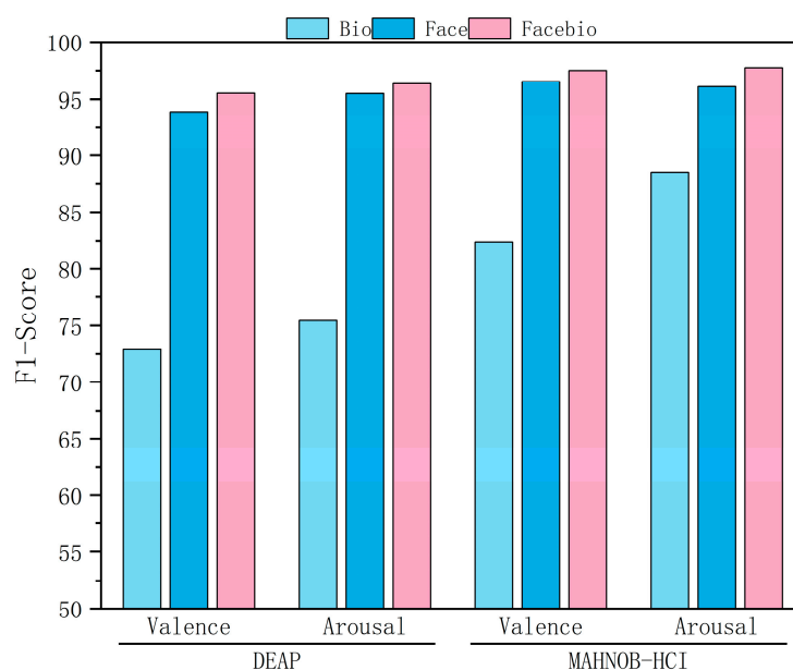
Figure 5. Classification results of ablation experiments (F1-Score).
