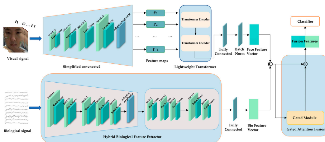
Figure 1. The overall architecture of the proposed Gated Biological Visual Network (GBV-Net).
