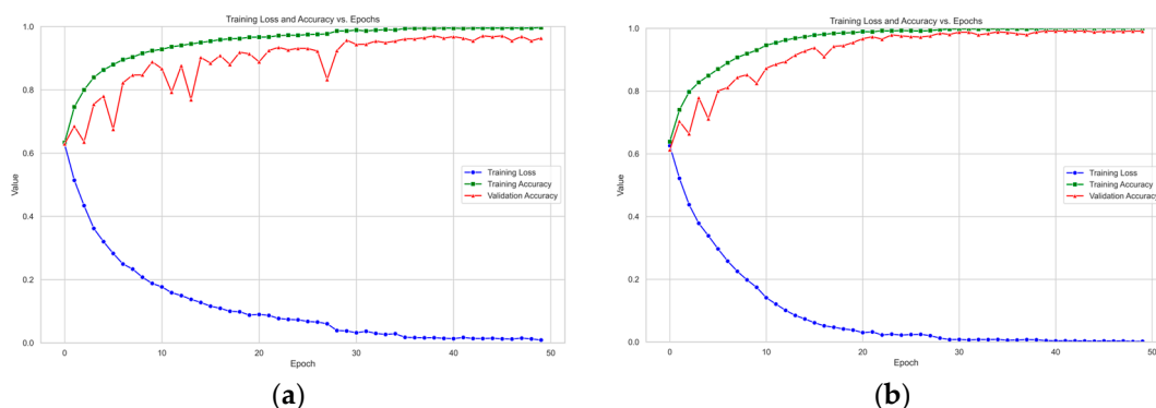
Figure 3. Model performance evaluation curves in the MAHNOB-HCI dataset. Here, (a) represents the Valence dimension curve and (b) represents the Arousal dimension curve.
