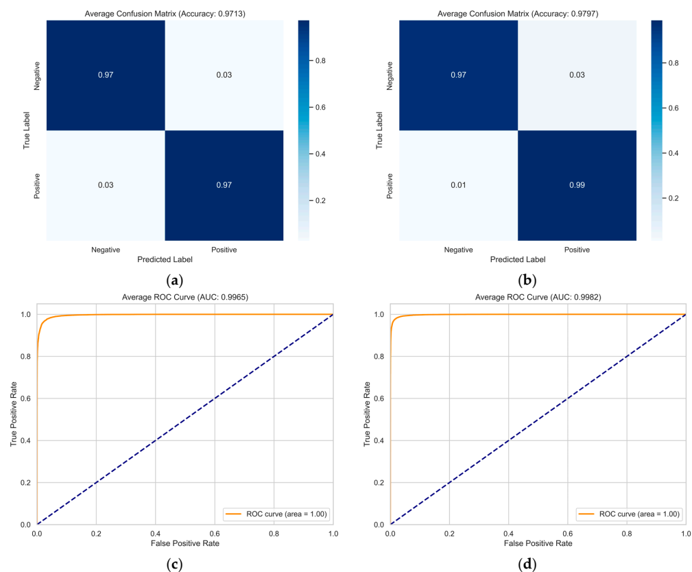
Figure 6. Classification average confusion matrix for the DEAP dataset on the (a) valence and (b) arousal dimensions ROC curves for the (c) valence and (d) arousal dimensions.
